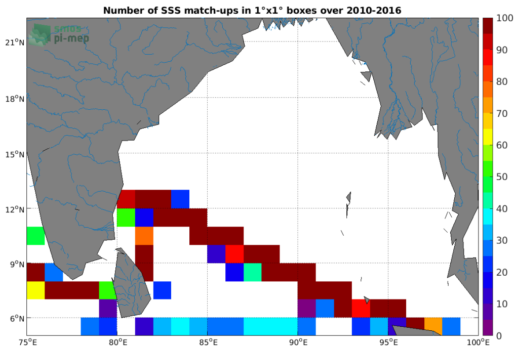
Figure 4: Number of SSS match-ups between TSG (LEGOS-DM) SSS and the CCI SSS L4 Merged-OI v2.31 - 30-day running (ESA) SSS product for the Ganga and Brahmaputra river plumes Pi-MEP region over 1°x1° boxes and for the full satellite product period.
