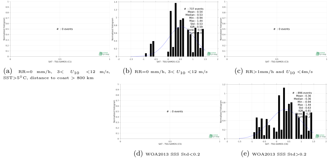
Figure 13: Normalized histogram of \Delta SSS (CCI L4 Merged-OI v1.8 - 7-day running (ESA) - TSG-SAMOS) for 5 different subdatasets corresponding to: RR=0 mm/h, 3 < U_{10} < 12 m/s, SST>5°C, distance to coast > 800 km (a), RR=0 mm/h, 3 < U_{10} < 12 m/s (b), RR>1mm/h and U_{10} < 4 m/s (c), WOA2013 SSS Std<0.2 (d), WOA2013 SSS Std>0.2 (e).
