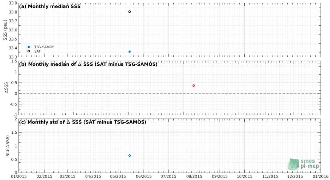
Figure 7: Time series of the monthly median SSS (top), median of \Delta\text{SSS} (Satellite - TSG-SAMOS) and Std of \Delta\text{SSS} (Satellite - TSG-SAMOS) over the Ganga and Brahmaputra river plumes Pi-MEP region considering all match-ups collected by the Pi-MEP.
