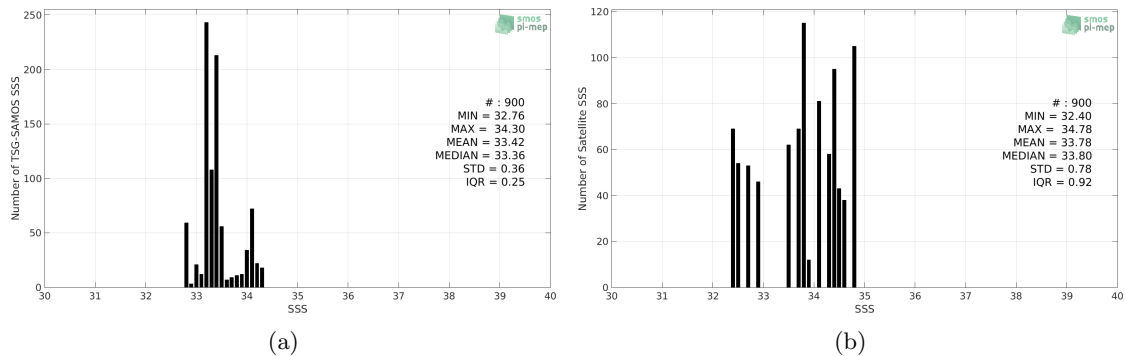
Figure 2: Histograms of SSS from TSG-SAMOS (a) and CCI L4 Merged-OI v1.8 - 7-day running (ESA) (b) considering all match-up pairs per bins of 0.1 over the Ganga and Brahmaputra river plumes Pi-MEP region and for the full satellite product period.
