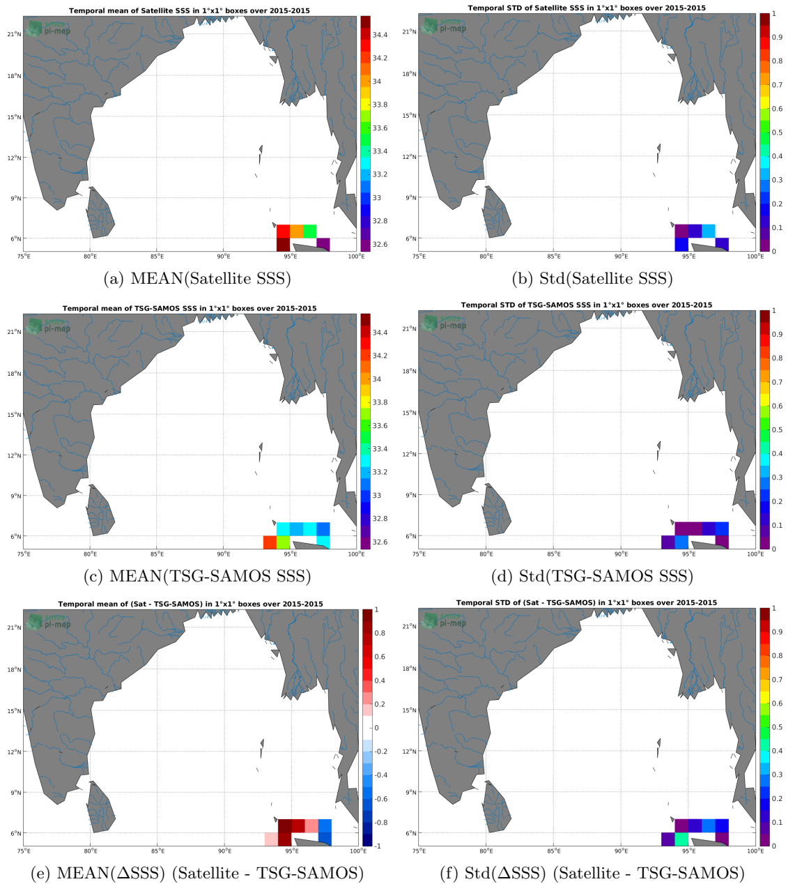
Figure 6: Temporal mean (left) and Std (right) of SSS from CCI L4 Merged-OI v1.8 - 7-day running (ESA) (top), TSG-SAMOS (middle), and of \Delta SSS (Satellite - TSG-SAMOS). Only match-up pairs are used to generate these maps.
