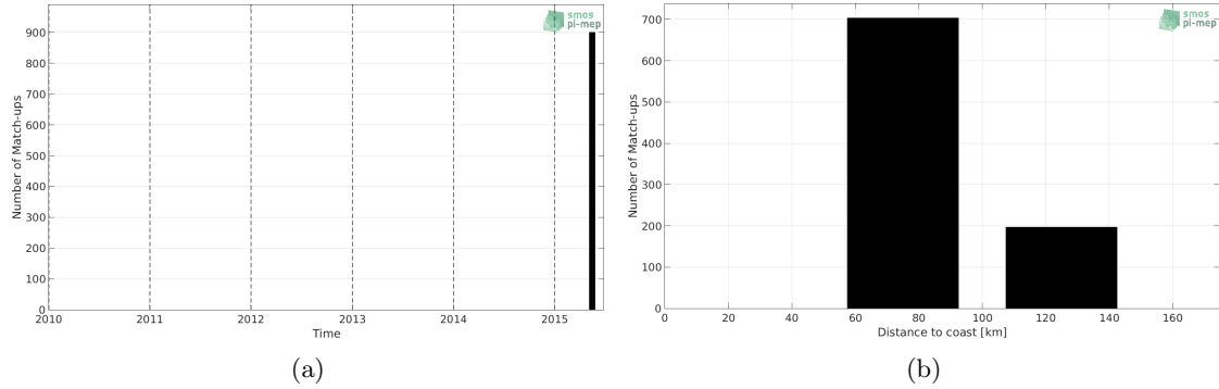
Figure 1: Number of match-ups between TSG-SAMOS and CCI-L4-ESA-MERGED-OI-V1.8-7DAY-RUNNING SSS as a function of time (a) and as function of the distance to coast (b) over the Ganga and Brahmaputra river plumes Pi-MEP region and for the full satellite product period.
