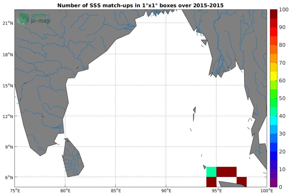
Figure 4: Number of SSS match-ups between TSG-SAMOS SSS and the CCI-L4-ESA-MERGED-OI-V1.8-7DAY-RUNNING SSS product for the Ganga and Brahmaputra river plumes Pi-MEP region over 1^\circ \times 1^\circ boxes and for the full satellite product period.
