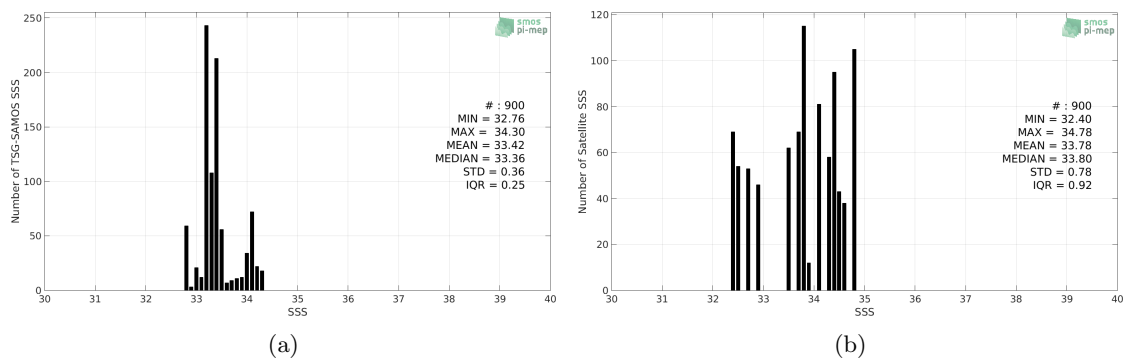
Figure 2: Histograms of SSS from TSG-SAMOS (a) and CCI-L4-ESA-MERGED-OI-V1.8-7DAY-RUNNING (b) considering all match-up pairs per bins of 0.1 over the Ganga and Brahmaputra river plumes Pi-MEP region and for the full satellite product period.
