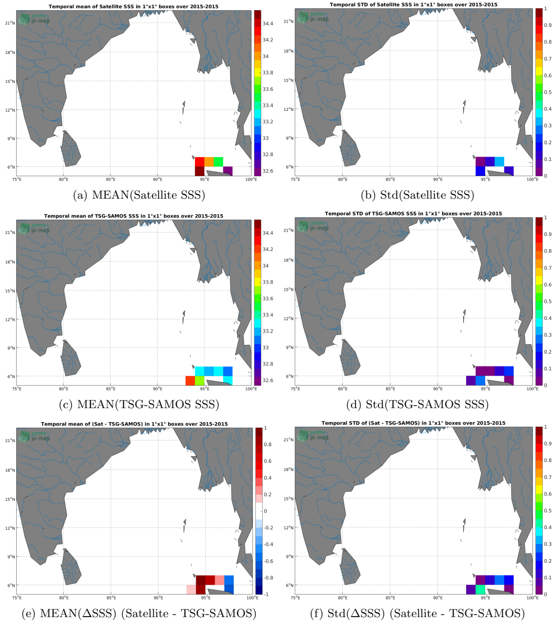
Figure 6: Temporal mean (left) and Std (right) of SSS from CCI-L4-ESA-MERGED-OI-V1.8-7DAY-RUNNING (top), TSG-SAMOS (middle), and of \Delta SSS (Satellite - TSG-SAMOS). Only match-up pairs are used to generate these maps.
