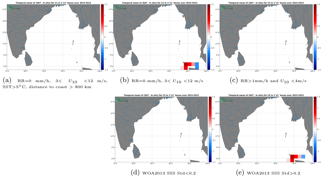
Figure 12: Temporal mean gridded over spatial boxes of size 1^\circ \times 1^\circ of \Delta SSS (CCI-L4-ESA-MERGED-OI-V1.8-7DAY-RUNNING - TSG-SAMOS) for 5 different subdatasets corresponding to:RR=0 mm/h, 3 < U_{10} < 12 m/s, SST >5^\circ C, distance to coast > 800 km (a), RR=0 mm/h, 3 < U_{10} < 12 m/s (b), RR >1 mm/h and U_{10} < 4 m/s (c), WOA2013 SSS Std <0.2 (d), WOA2013 SSS Std >0.2 (e).
