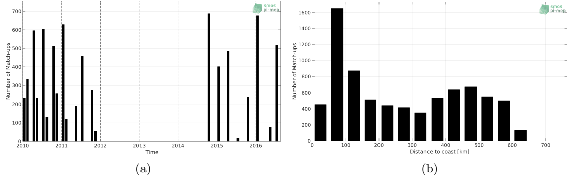
Figure 1: Number of match-ups between TSG-LEGOS-DM and CCI L4 Merged-OI v1.8 - 7-day running (ESA) SSS as a function of time (a) and as function of the distance to coast (b) over the Ganga and Brahmaputra river plumes Pi-MEP region and for the full satellite product period.
