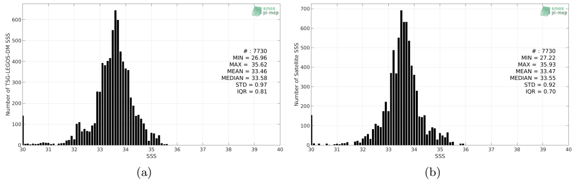
Figure 2: Histograms of SSS from TSG-LEGOS-DM (a) and CCI L4 Merged-OI v1.8 - 7-day running (ESA) (b) considering all match-up pairs per bins of 0.1 over the Ganga and Brahmaputra river plumes Pi-MEP region and for the full satellite product period.
