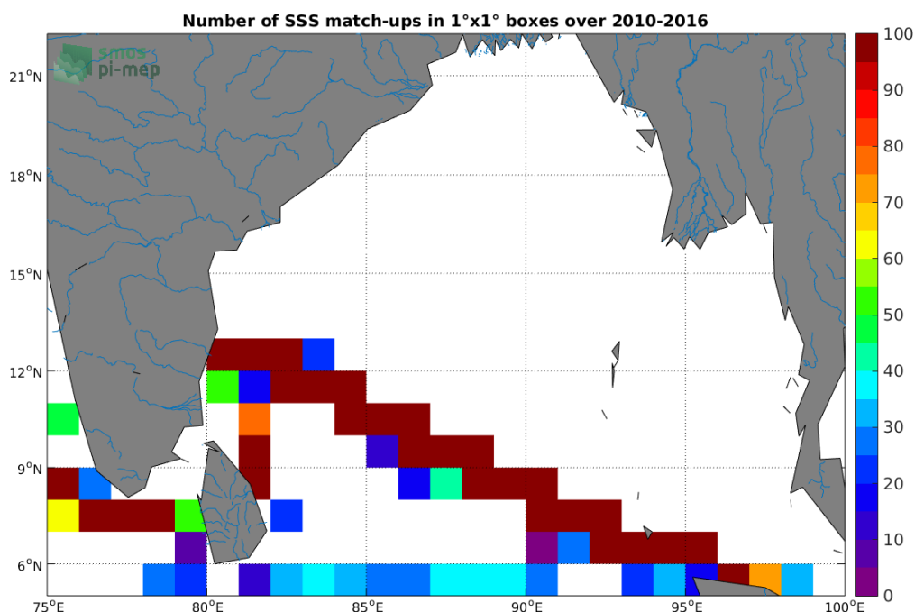
Figure 4: Number of SSS match-ups between TSG-LEGOS-DM SSS and the CCI L4 Merged-OI v1.8 - 7-day running (ESA) SSS product for the Ganga and Brahmaputra river plumes Pi-MEP region over 1°x1° boxes and for the full satellite product period.
