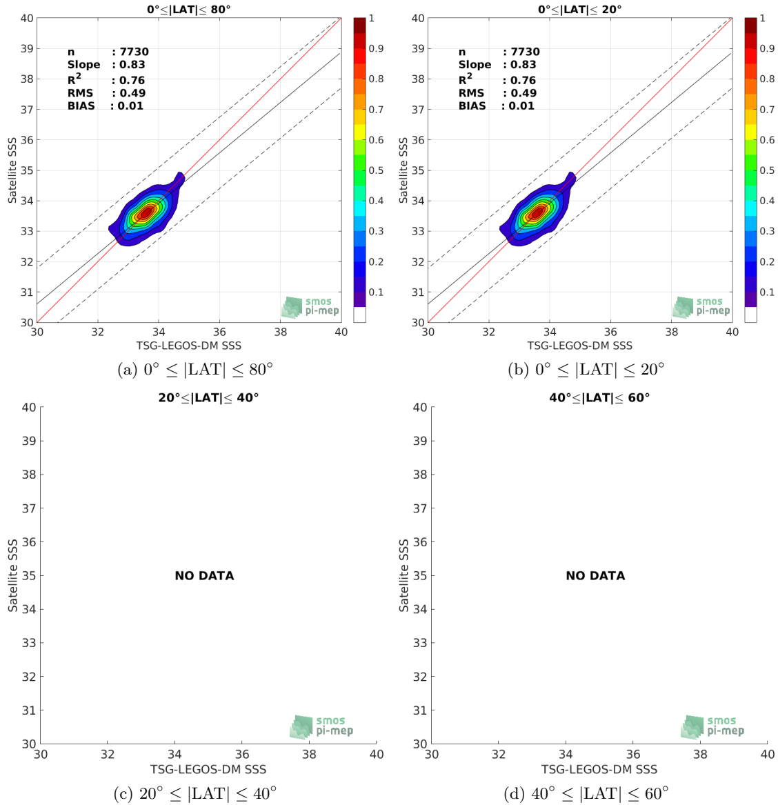
Figure 9: Contour maps of the concentration of CCI-L4-ESA-MERGED-OI-V1.8-7DAY-RUNNING SSS (y-axis) versus TSG-LEGOS-DM SSS (x-axis) at match-up pairs for different latitude bands. For each plot, the red line shows x=y . The black thin and dashed lines indicate a linear fit through the data cloud and the \pm 95\% confidence levels, respectively. The number match-up pairs n , the slope and R^2 coefficient of the linear fit, the root mean square (RMS) and the mean bias between satellite and in situ data are indicated for each latitude band in each plots.
