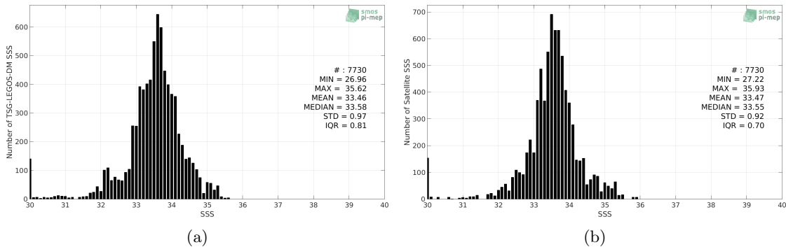
Figure 2: Histograms of SSS from TSG-LEGOS-DM (a) and CCI-L4-ESA-MERGED-OI-V1.8-7DAY-RUNNING (b) considering all match-up pairs per bins of 0.1 over the Ganga and Brahmaputra river plumes Pi-MEP region and for the full satellite product period.
