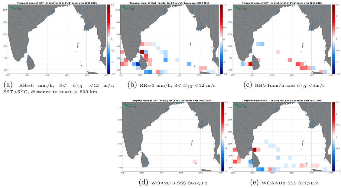
Figure 12: Temporal mean gridded over spatial boxes of size 1^\circ \times 1^\circ of \Delta SSS (CCI-L4-ESA-MERGED-OI-V1.8-7DAY-RUNNING - TSG-LEGOS-DM) for 5 different subdatasets corresponding to:RR=0 mm/h, 3 < U_{10} < 12 m/s, SST >5^\circ C, distance to coast > 800 km (a), RR=0 mm/h, 3 < U_{10} < 12 m/s (b), RR >1 mm/h and U_{10} < 4 m/s (c), WOA2013 SSS Std <0.2 (d), WOA2013 SSS Std >0.2 (e).
