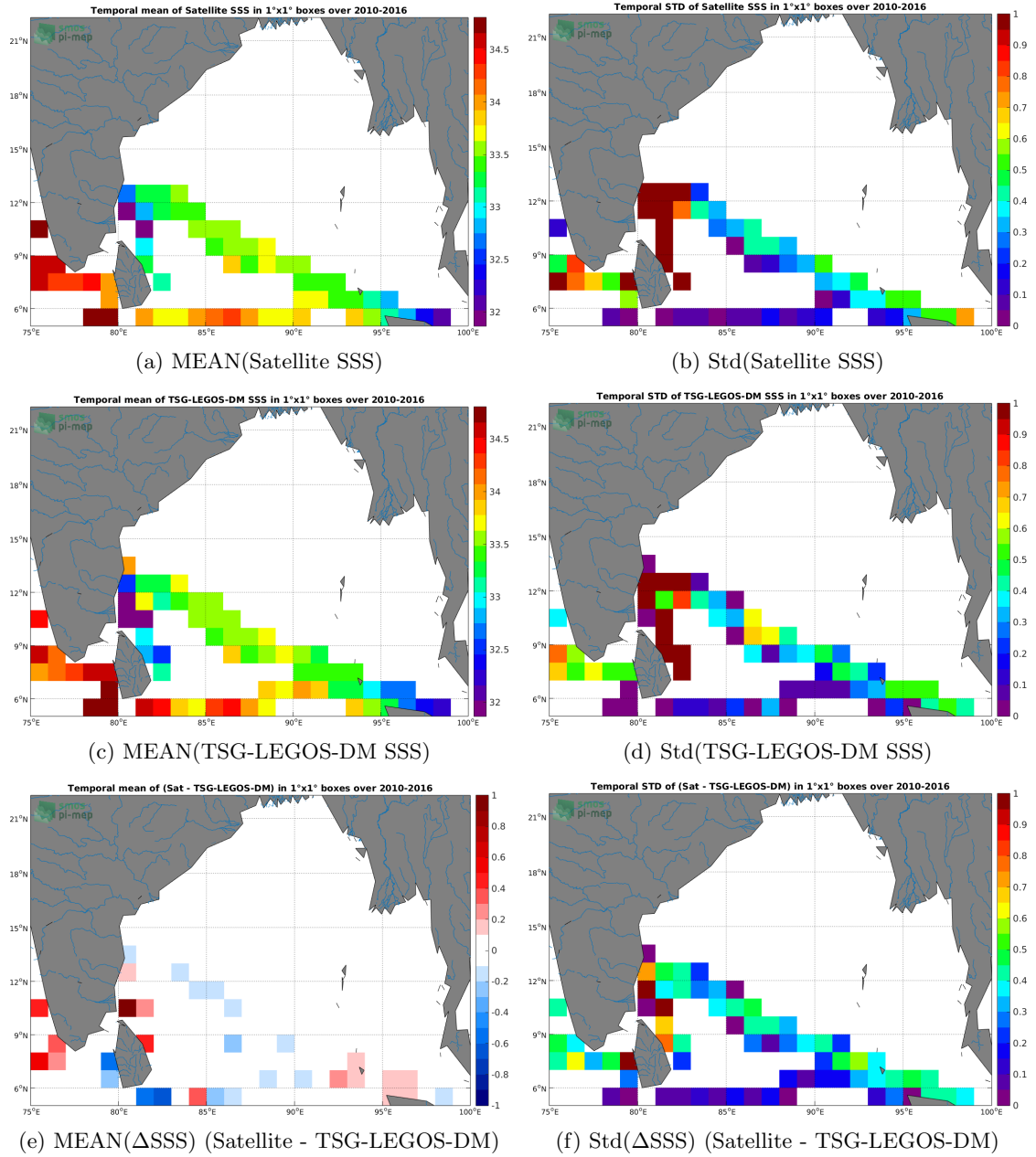
Figure 6: Temporal mean (left) and Std (right) of SSS from CCI-L4-ESA-MERGED-OI-V1.8-7DAY-RUNNING (top), TSG-LEGOS-DM (middle), and of \Delta SSS (Satellite - TSG-LEGOS-DM). Only match-up pairs are used to generate these maps.
