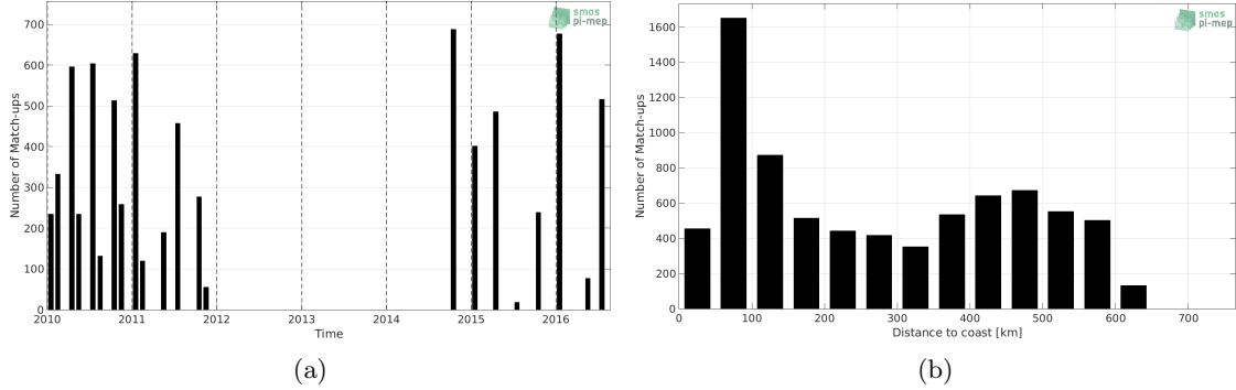
Figure 1: Number of match-ups between TSG-LEGOS-DM and CCI-L4-ESA-MERGED-OI-V1.8-7DAY-RUNNING SSS as a function of time (a) and as function of the distance to coast (b) over the Ganga and Brahmaputra river plumes Pi-MEP region and for the full satellite product period.
