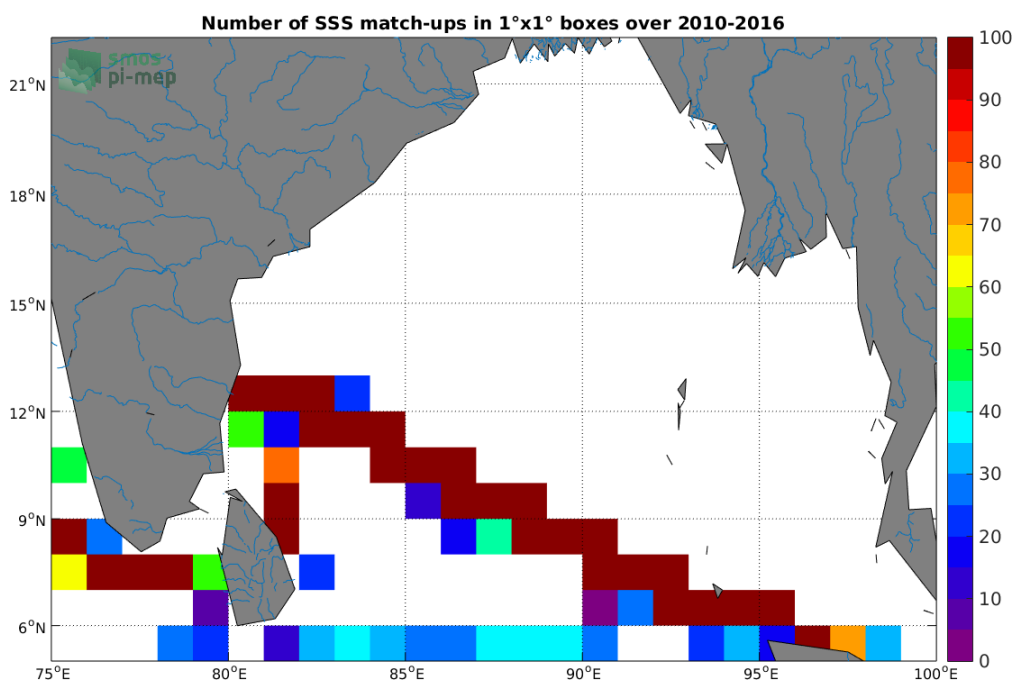
Figure 4: Number of SSS match-ups between TSG-LEGOS-DM SSS and the CCI-L4-ESA-MERGED-OI-V1.8-7DAY-RUNNING SSS product for the Ganga and Brahmaputra river plumes Pi-MEP region over 1°x1° boxes and for the full satellite product period.
