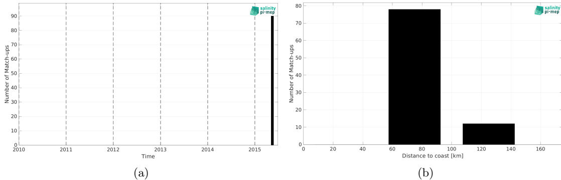
Figure 2: Number of match-ups between TSG (SAMOS) and Aquarius SSS L4 OI v5 - Weekly (IPRC) SSS as a function of time (a) and as function of the distance to coast (b) over the Ganga and Brahmaputra river plumes Pi-MEP region and for the full satellite product period.
