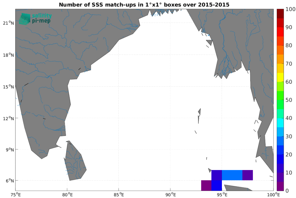
Figure 5: Number of SSS match-ups between TSG (SAMOS) SSS and the Aquarius SSS L4 OI v5 - Weekly (IPRC) SSS product for the Ganga and Brahmaputra river plumes Pi-MEP region over 1°×1° boxes and for the full satellite product period.
