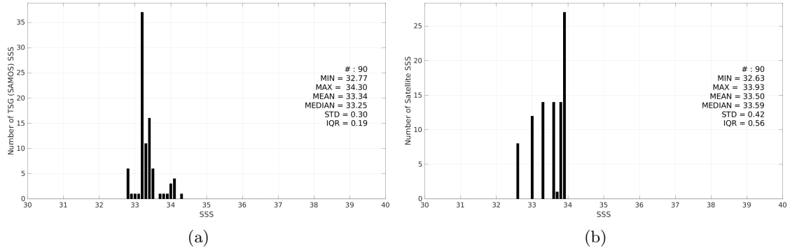
Figure 3: Histograms of SSS from TSG (SAMOS) (a) and Aquarius SSS L4 OI v5 - Weekly (IPRC) (b) considering all match-up pairs per bins of 0.1 over the Ganga and Brahmaputra river plumes Pi-MEP region and for the full satellite product period.
