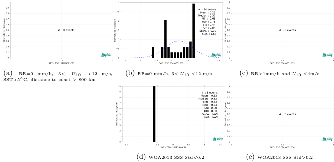
Figure 15: Normalized histogram of \Delta SSS (Aquarius SSS L4 OI v5 - Weekly (IPRC) - TSG (SAMOS)) for 5 different subdatasets corresponding to: RR=0 mm/h, 3 < U_{10} < 12 m/s, SST > 5°C, distance to coast > 800 km (a), RR=0 mm/h, 3 < U_{10} < 12 m/s (b), RR > 1mm/h and U_{10} < 4 m/s (c), WOA2013 SSS Std < 0.2 (d), WOA2013 SSS Std > 0.2 (e).
