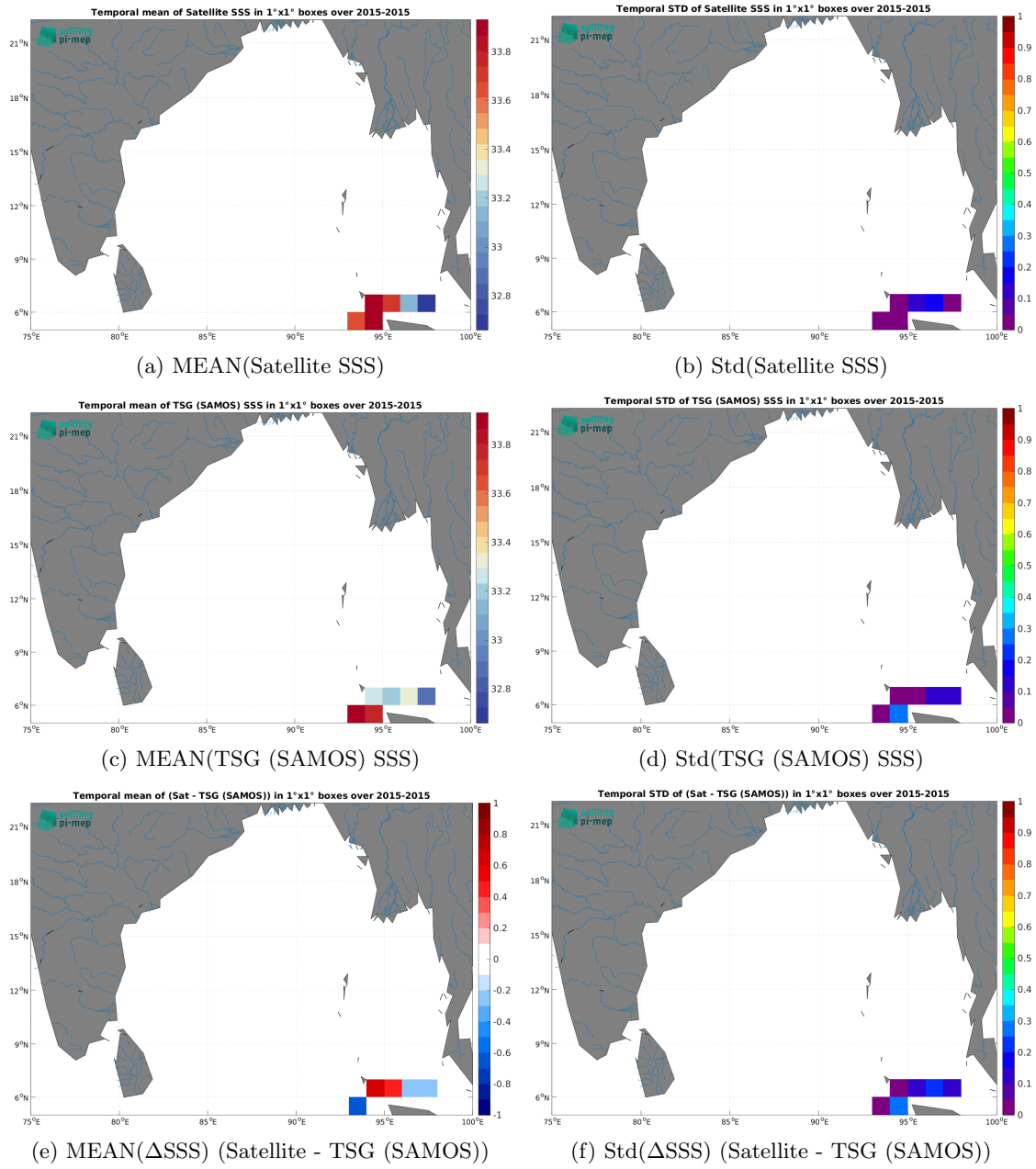
Figure 7: Temporal mean (left) and Std (right) of SSS from Aquarius SSS L4 OI v5 - Weekly (IPRC) (top), TSG (SAMOS) (middle), and of \Delta SSS (Satellite - TSG (SAMOS)). Only match-up pairs are used to generate these maps.
