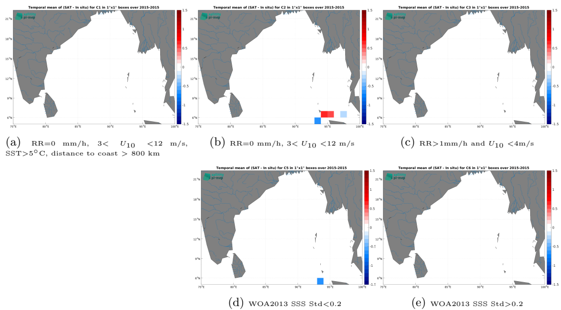
Figure 14: Temporal mean gridded over spatial boxes of size 1^\circ \times 1^\circ of \Delta SSS (Aquarius SSS L4 OI v5 - Weekly (IPRC) - TSG (SAMOS)) for 5 different subdatasets corresponding to:RR=0 mm/h, 3 < U_{10} < 12 m/s, SST >5^\circ C, distance to coast > 800 km (a), RR=0 mm/h, 3 < U_{10} < 12 m/s (b), RR >1 mm/h and U_{10} < 4 m/s (c), WOA2013 SSS Std <0.2 (d), WOA2013 SSS Std >0.2 (e).
