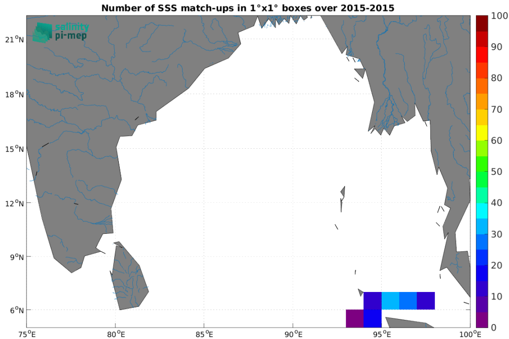
Figure 4: Number of SSS match-ups between TSG (SAMOS) SSS and the Aquarius SSS L4 OI v5 - Weekly (IPRC) SSS product for the Ganga and Brahmaputra river plumes Pi-MEP region over 1^{\circ} \times 1^{\circ} boxes and for the full satellite product period.
