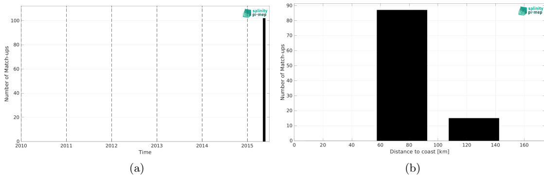
Figure 1: Number of match-ups between TSG (SAMOS) and Aquarius SSS L4 OI v5 - Weekly (IPRC) SSS as a function of time (a) and as function of the distance to coast (b) over the Ganga and Brahmaputra river plumes Pi-MEP region and for the full satellite product period.
