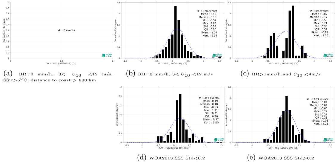
Figure 15: Normalized histogram of \Delta SSS (Aquarius SSS L4 OI v5 - Weekly (IPRC) - TSG (LEGOS-DM)) for 5 different subdatasets corresponding to: RR=0 mm/h, 3 < U_{10} < 12 m/s, SST >5^{\circ} C, distance to coast > 800 km (a), RR=0 mm/h, 3 < U_{10} < 12 m/s (b), RR >1 mm/h and U_{10} < 4 m/s (c), WOA2013 SSS Std <0.2 (d), WOA2013 SSS Std >0.2 (e).
