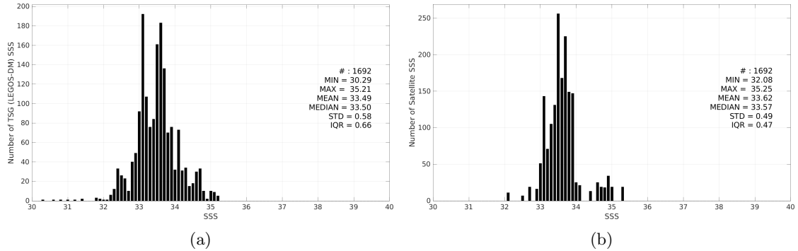
Figure 3: Histograms of SSS from TSG (LEGOS-DM) (a) and Aquarius SSS L4 OI v5 - Weekly (IPRC) (b) considering all match-up pairs per bins of 0.1 over the Ganga and Brahmaputra river plumes Pi-MEP region and for the full satellite product period.
