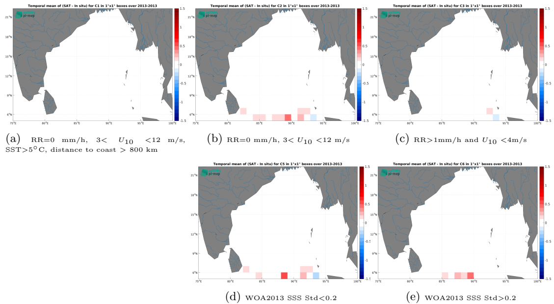
Figure 13: Temporal mean gridded over spatial boxes of size 1^\circ \times 1^\circ of \Delta SSS (Aquarius SSS L4 OI v5 - Weekly (IPRC) - Surface drifters) for 5 different subdatasets corresponding to:RR=0 mm/h, 3 < U_{10} < 12 m/s, SST > 5^\circ\text{C} , distance to coast > 800 km (a), RR=0 mm/h, 3 < U_{10} < 12 m/s (b), RR > 1 mm/h and U_{10} < 4 m/s (c), WOA2013 SSS Std < 0.2 (d), WOA2013 SSS Std > 0.2 (e).
