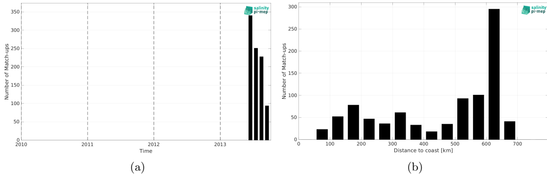
Figure 2: Number of match-ups between Surface drifters and Aquarius SSS L4 OI v5 - Weekly (IPRC) SSS as a function of time (a) and as function of the distance to coast (b) over the Ganga and Brahmaputra river plumes Pi-MEP region and for the full satellite product period.
