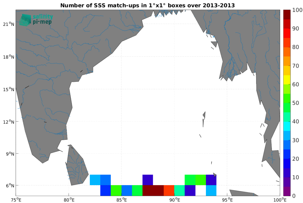
Figure 4: Number of SSS match-ups between Surface drifters SSS and the Aquarius SSS L4 OI v5 - Weekly (IPRC) SSS product for the Ganga and Brahmaputra river plumes Pi-MEP region over 1^\circ \times 1^\circ boxes and for the full satellite product period.
