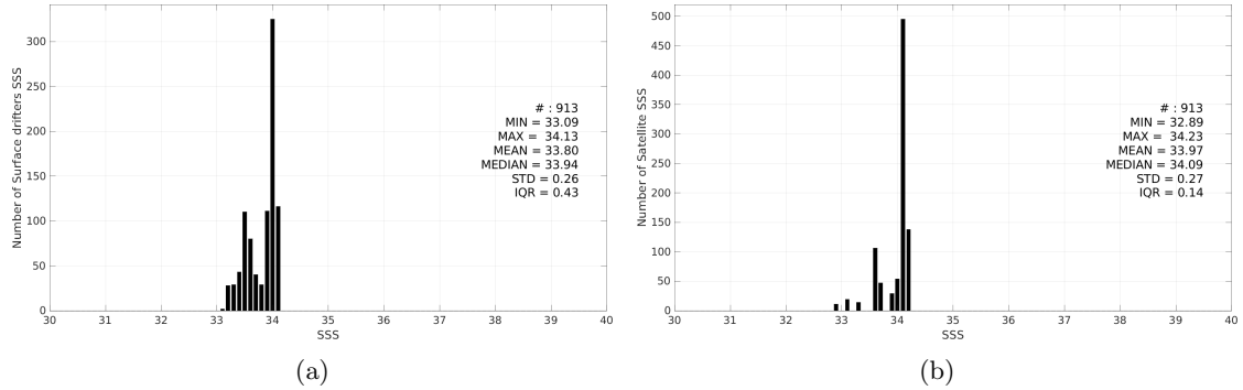
Figure 3: Histograms of SSS from Surface drifters (a) and Aquarius SSS L4 OI v5 - Weekly (IPRC) (b) considering all match-up pairs per bins of 0.1 over the Ganga and Brahmaputra river plumes Pi-MEP region and for the full satellite product period.
