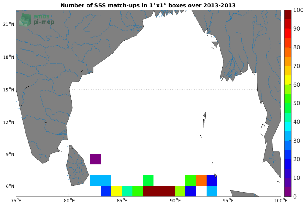
Figure 3: Number of SSS match-ups between Surface drifters SSS and the Aquarius SSS L4 OI v5 - Weekly (IPRC) SSS product for the Ganga and Brahmaputra river plumes Pi-MEP region over 1°x1° boxes and for the full satellite product period.
