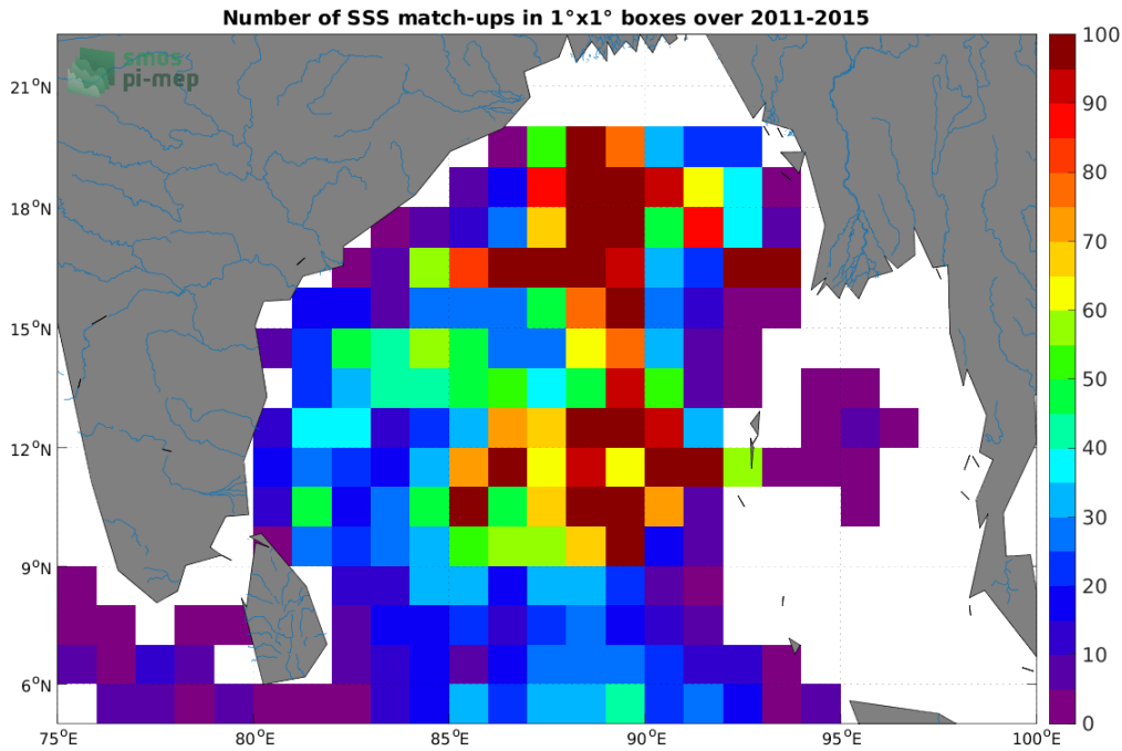
Figure 4: Number of SSS match-ups between Argo SSS and the Aquarius SSS L4 OI v5 - Weekly (IPRC) SSS product for the Ganga and Brahmaputra river plumes Pi-MEP region over 1^{\circ} \times 1^{\circ} boxes and for the full satellite product period.
