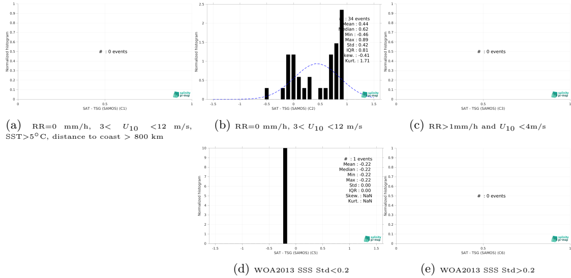
Figure 15: Normalized histogram of \Delta SSS (Aquarius SSS L4 OI v5 - Monthly (IPRC) - TSG (SAMOS)) for 5 different subdatasets corresponding to: RR=0 mm/h, 3 < U_{10} < 12 m/s, SST > 5°C, distance to coast > 800 km (a), RR=0 mm/h, 3 < U_{10} < 12 m/s (b), RR > 1mm/h and U_{10} < 4 m/s (c), WOA2013 SSS Std < 0.2 (d), WOA2013 SSS Std > 0.2 (e).
