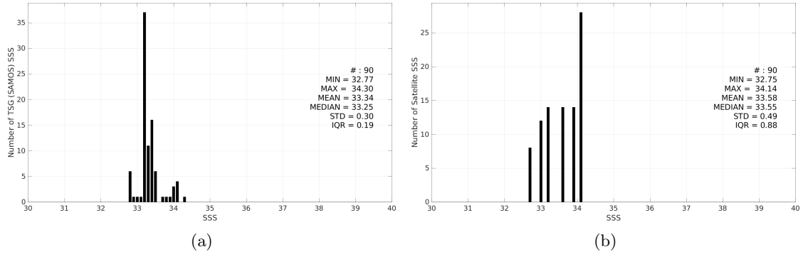
Figure 3: Histograms of SSS from TSG (SAMOS) (a) and Aquarius SSS L4 OI v5 - Monthly (IPRC) (b) considering all match-up pairs per bins of 0.1 over the Ganga and Brahmaputra river plumes Pi-MEP region and for the full satellite product period.
