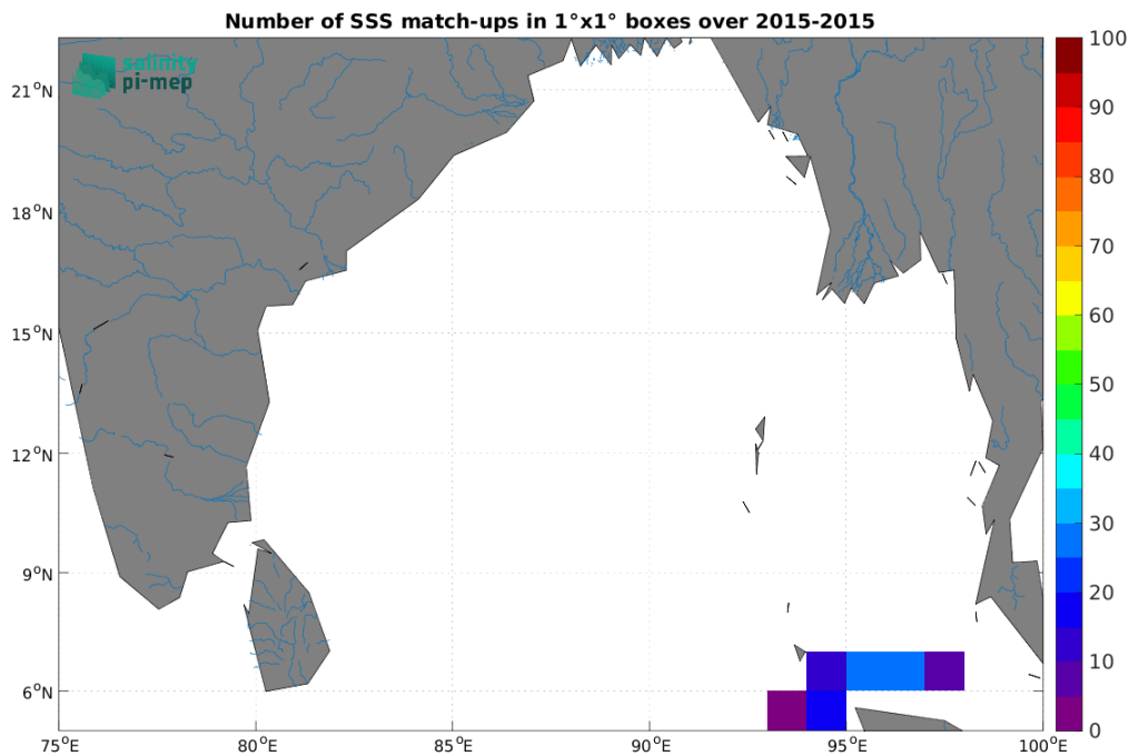
Figure 5: Number of SSS match-ups between TSG (SAMOS) SSS and the Aquarius SSS L4 OI v5 - Monthly (IPRC) SSS product for the Ganga and Brahmaputra river plumes Pi-MEP region over 1^\circ \times 1^\circ boxes and for the full satellite product period.
