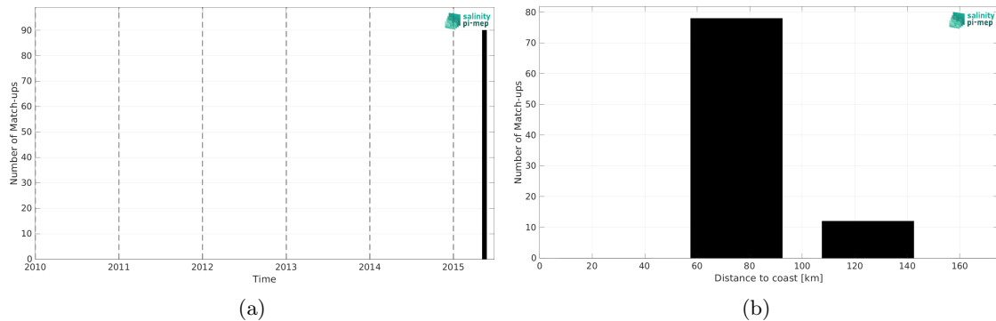
Figure 2: Number of match-ups between TSG (SAMOS) and Aquarius SSS L4 OI v5 - Monthly (IPRC) SSS as a function of time (a) and as function of the distance to coast (b) over the Ganga and Brahmaputra river plumes Pi-MEP region and for the full satellite product period.
