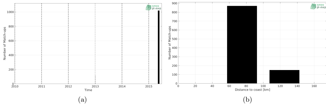
Figure 1: Number of match-ups between TSG (SAMOS) and Aquarius SSS L4 OI v5 - Monthly (IPRC) SSS as a function of time (a) and as function of the distance to coast (b) over the Ganga and Brahmaputra river plumes Pi-MEP region and for the full satellite product period.
