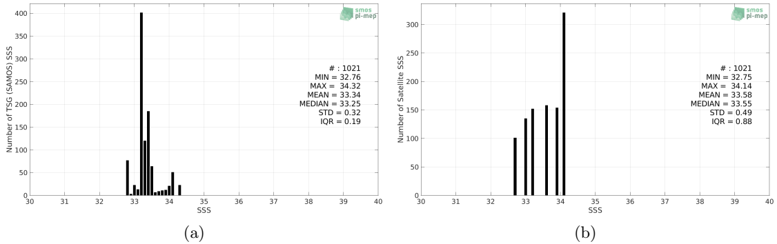
Figure 2: Histograms of SSS from TSG (SAMOS) (a) and Aquarius SSS L4 OI v5 - Monthly (IPRC) (b) considering all match-up pairs per bins of 0.1 over the Ganga and Brahmaputra river plumes Pi-MEP region and for the full satellite product period.
