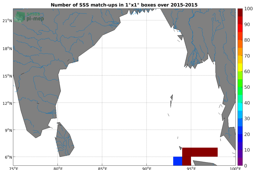
Figure 4: Number of SSS match-ups between TSG (SAMOS) SSS and the Aquarius SSS L4 OI v5 - Monthly (IPRC) SSS product for the Ganga and Brahmaputra river plumes Pi-MEP region over 1^{\circ} \times 1^{\circ} boxes and for the full satellite product period.
