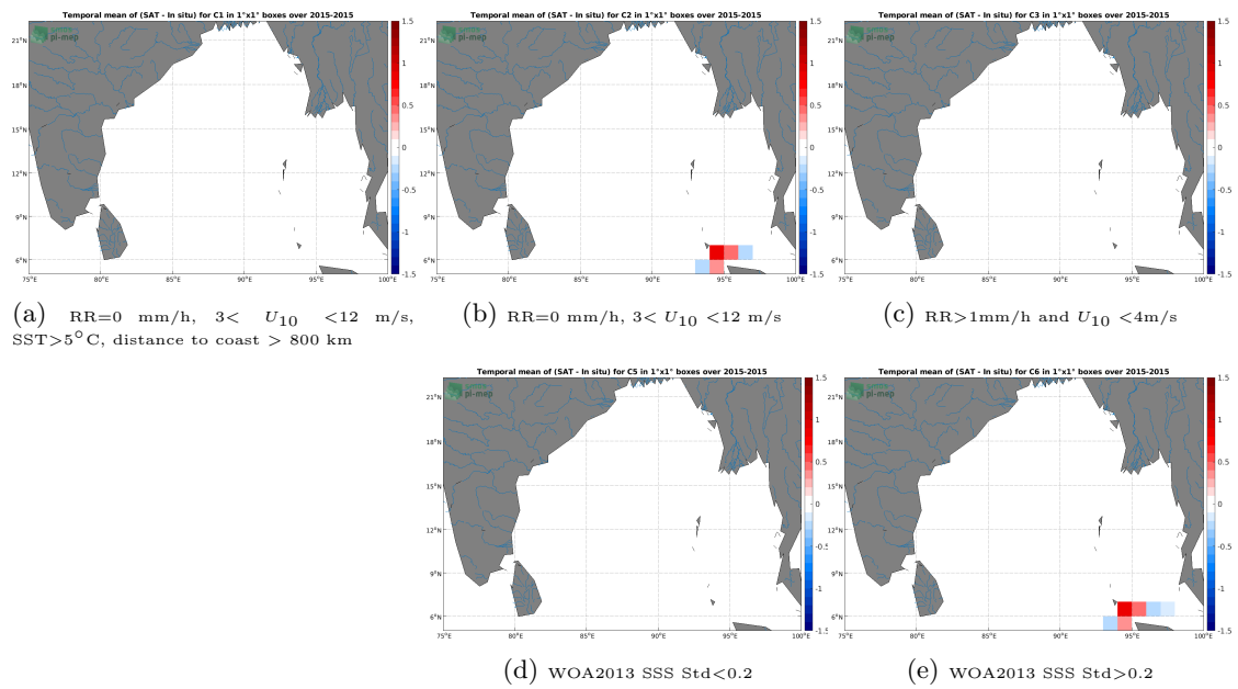
Figure 12: Temporal mean gridded over spatial boxes of size 1°x1° of \Delta SSS (Aquarius SSS L4 OI v5 - Monthly (IPRC) - TSG (SAMOS)) for 5 different subdatasets corresponding to:RR=0 mm/h, 3 < U_{10} < 12 m/s, SST>5°C, distance to coast > 800 km (a), RR=0 mm/h, 3 < U_{10} < 12 m/s (b), RR>1mm/h and U_{10} < 4 m/s (c), WOA2013 SSS Std<0.2 (d), WOA2013 SSS Std>0.2 (e).
