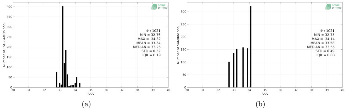
Figure 2: Histograms of SSS from TSG-SAMOS (a) and Aquarius-L4-IPRC-V5-MONTHLY (b) considering all match-up pairs per bins of 0.1 over the Ganga and Brahmaputra river plumes Pi-MEP region and for the full satellite product period.
