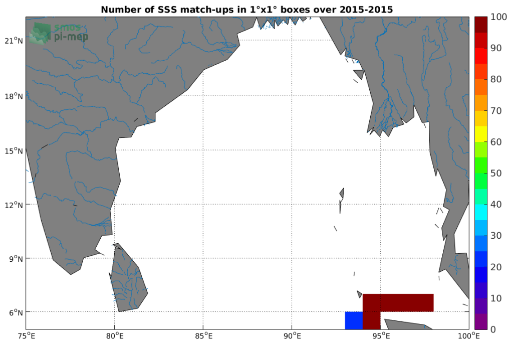
Figure 4: Number of SSS match-ups between TSG-SAMOS SSS and the Aquarius-L4-IPRC-V5-MONTHLY SSS product for the Ganga and Brahmaputra river plumes Pi-MEP region over 1°x1° boxes and for the full satellite product period.
