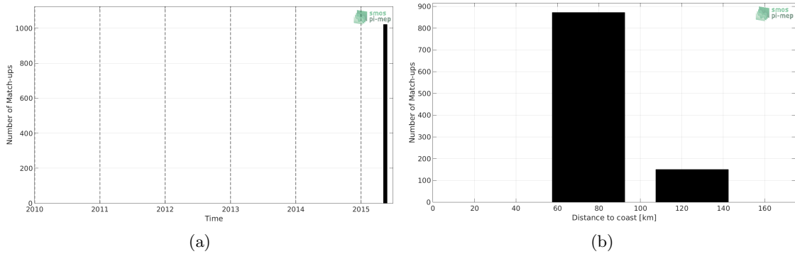
Figure 1: Number of match-ups between TSG-SAMOS and Aquarius-L4-IPRC-V5-MONTHLY SSS as a function of time (a) and as function of the distance to coast (b) over the Ganga and Brahmaputra river plumes Pi-MEP region and for the full satellite product period.
