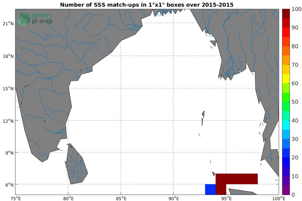
Figure 4: Number of SSS match-ups between TSG-SAMOS SSS and the Aquarius-L4-IPRC-V5-MONTHLY SSS product for the Ganga and Brahmaputra river plumes Pi-MEP region over 1^\circ \times 1^\circ boxes and for the full satellite product period.
