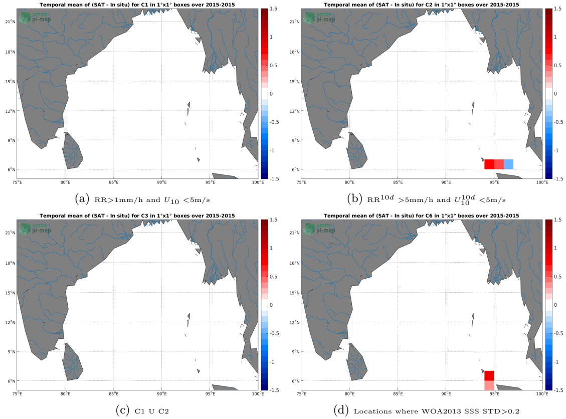
Figure 12: Temporal mean gridded over spatial boxes of size 1^\circ \times 1^\circ of \Delta SSS (Aquarius-L4-IPRC-V5-MONTHLY - TSG-SAMOS) for 4 different subdatasets corresponding to: RR > 1mm/h and U_{10} < 5\text{m/s} (a), RR^{10d} > 5\text{mm/h} and U_{10}^{10d} < 5\text{m/s} (b), C1 U C2 (c), Locations where WOA2013 SSS STD > 0.2 (d).
