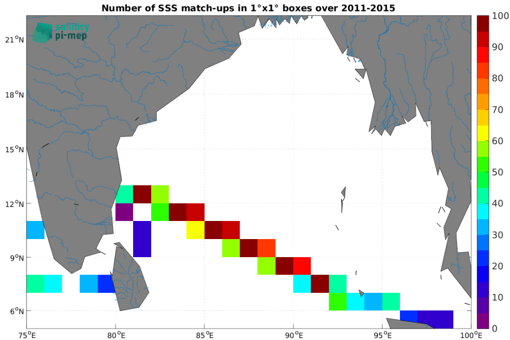
Figure 4: Number of SSS match-ups between TSG (LEGOS-DM) SSS and the Aquarius SSS L4 OI v5 - Monthly (IPRC) SSS product for the Ganga and Brahmaputra river plumes Pi-MEP region over 1^\circ \times 1^\circ boxes and for the full satellite product period.
