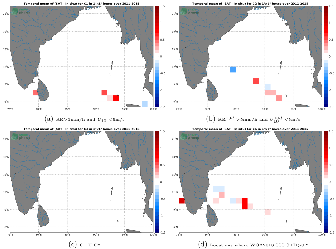
Figure 12: Temporal mean gridded over spatial boxes of size 1^\circ \times 1^\circ of \Delta SSS (Aquarius-L4-IPRC-V5-MONTHLY - TSG-LEGOS-DM) for 4 different subdatasets corresponding to: RR > 1 mm/h and U_{10} < 5 m/s (a), RR 10d > 5 mm/h and U_{10}^{10d} < 5 m/s (b), C1 U C2 (c), Locations where WOA2013 SSS STD > 0.2 (d).
