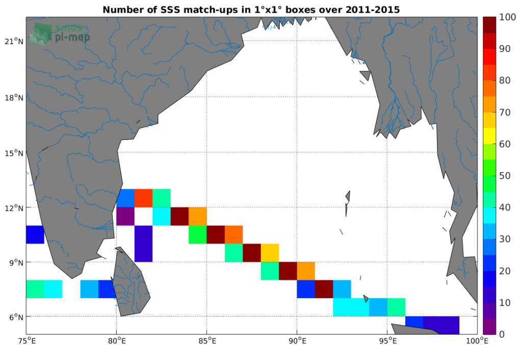
Figure 4: Number of SSS match-ups between TSG-LEGOS-DM SSS and the Aquarius-L4-IPRC-V5-MONTHLY SSS product for the Ganga and Brahmaputra river plumes Pi-MEP region over 1°x1° boxes and for the full satellite product period.
