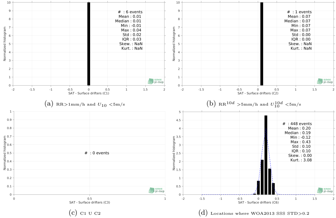
Figure 12: Normalized histogram of \Delta\text{SSS} (Aquarius-L4-IPRC-V5-MONTHLY - Surface drifters) for 6 different subdatasets corresponding to: RR > 1\text{mm/h} and U_{10} < 5\text{m/s} (a), RR^{10d} > 5\text{mm/h} and U_{10}^{10d} < 5\text{m/s} (b), C1 \cup C2 (c), Locations where WOA2013 SSS STD > 0.2 (d).
