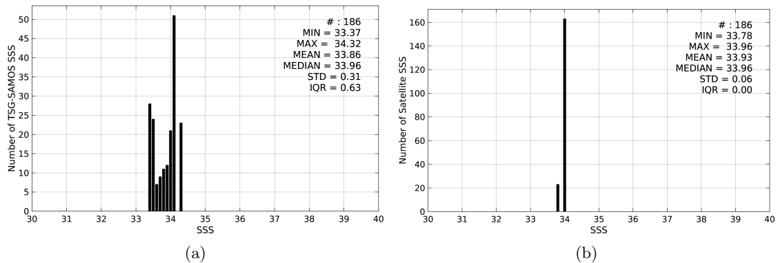
Figure 2: Histograms of SSS from TSG-SAMOS (a) and Aquarius-L4-IPRC-V4-WEEKLY (b) considering all match-up pairs per bins of 0.1 over the Ganga and Brahmaputra river plumes Pi-MEP region and for the full satellite product period.
