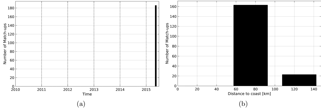
Figure 1: Number of match-ups between TSG-SAMOS and Aquarius-L4-IPRC-V4-WEEKLY SSS as a function of time (a) and as function of the distance to coast (b) over the Ganga and Brahmaputra river plumes Pi-MEP region and for the full satellite product period.
