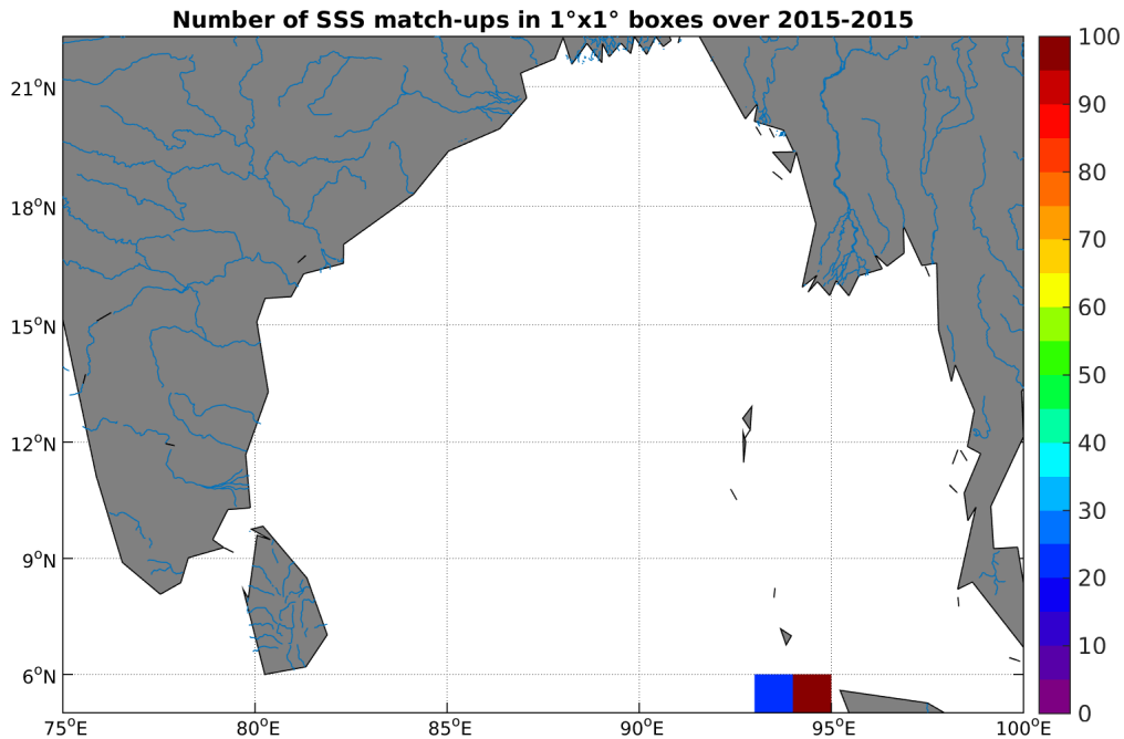
Figure 4: Number of SSS match-ups between TSG-SAMOS SSS and the Aquarius-L4-IPRC-V4-WEEKLY SSS product for the Ganga and Brahmaputra river plumes Pi-MEP region over 1^{\circ} \times 1^{\circ} boxes and for the full satellite product period.
