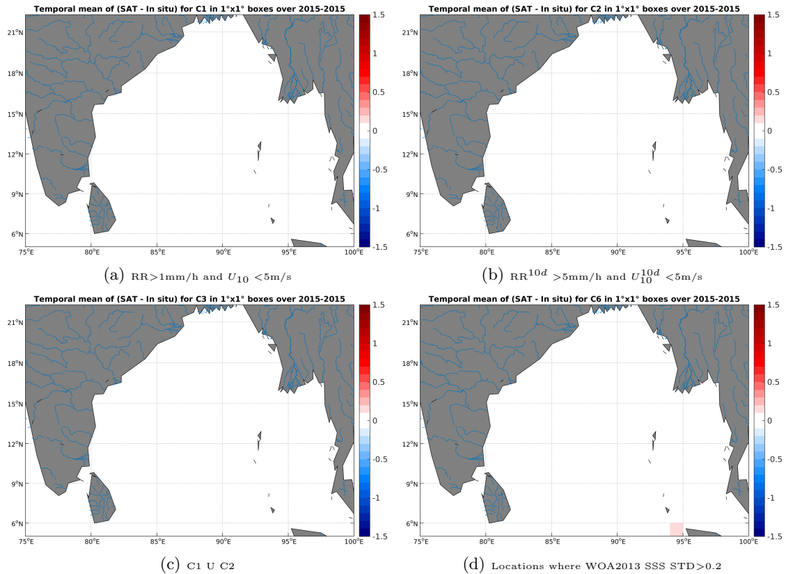
Figure 12: Temporal mean gridded over spatial boxes of size 1°x1° of \Delta SSS (Aquarius-L4-IPRC-V4-WEEKLY - TSG-SAMOS) for 4 different subdatasets corresponding to:RR>1mm/h and U_{10} < 5\text{m/s} (a), RR^{10d} > 5\text{mm/h} and U_{10}^{10d} < 5\text{m/s} (b), C1 U C2 (c),Locations where WOA2013 SSS STD>0.2 (d).
