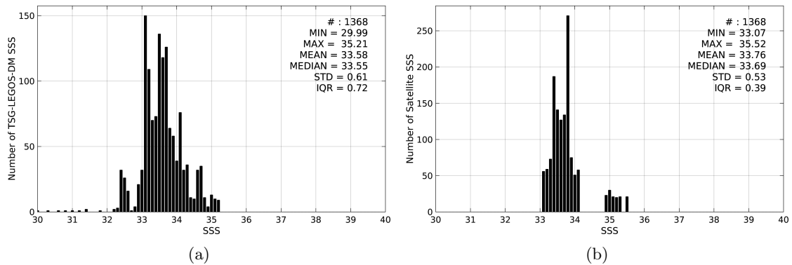
Figure 2: Histograms of SSS from TSG-LEGOS-DM (a) and Aquarius-L4-IPRC-V4-WEEKLY (b) considering all match-up pairs per bins of 0.1 over the Ganga and Brahmaputra river plumes Pi-MEP region and for the full satellite product period.
