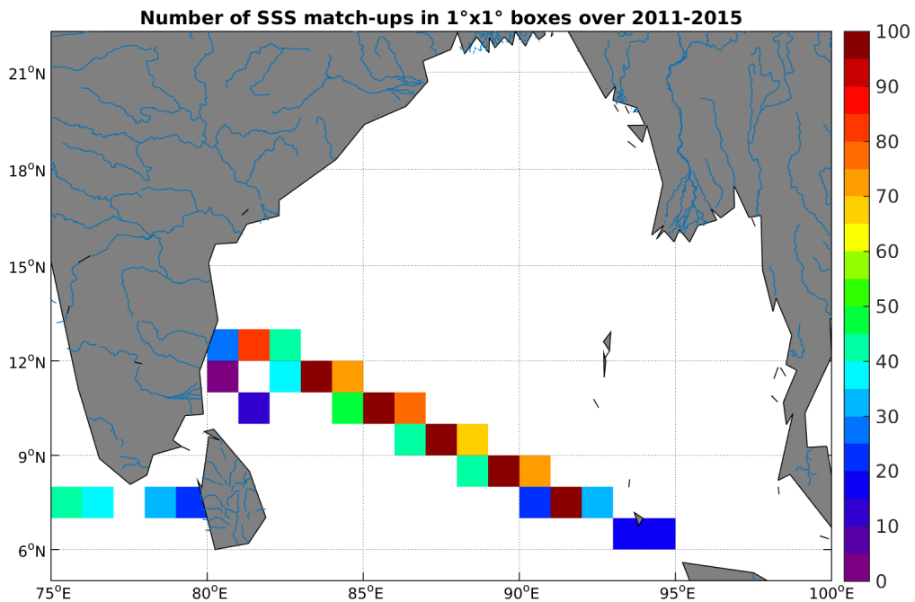
Figure 4: Number of SSS match-ups between TSG-LEGOS-DM SSS and the Aquarius-L4-IPRC-V4-WEEKLY SSS product for the Ganga and Brahmaputra river plumes Pi-MEP region over 1^{\circ} \times 1^{\circ} boxes and for the full satellite product period.
