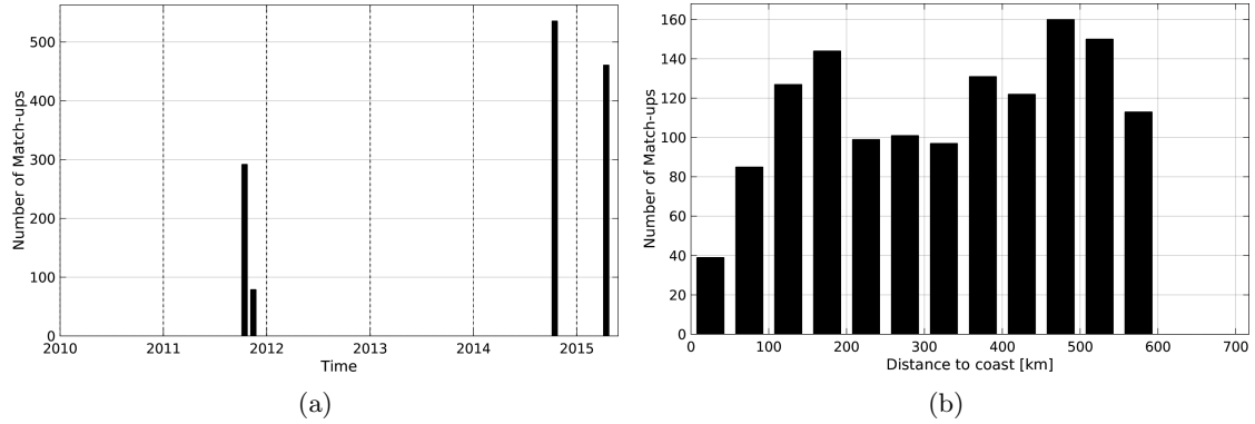
Figure 1: Number of match-ups between TSG-LEGOS-DM and Aquarius-L4-IPRC-V4-WEEKLY SSS as a function of time (a) and as function of the distance to coast (b) over the Ganga and Brahmaputra river plumes Pi-MEP region and for the full satellite product period.
