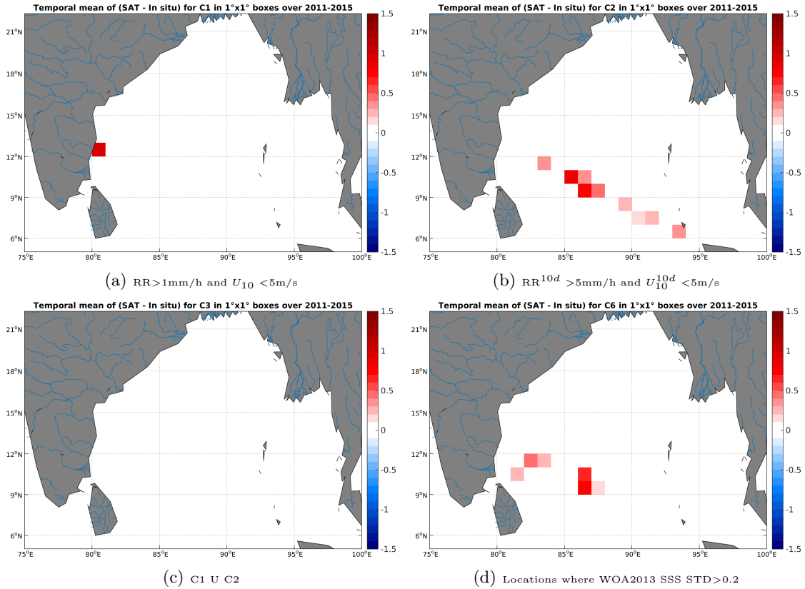
Figure 12: Temporal mean gridded over spatial boxes of size 1°x1° of \Delta SSS (Aquarius-L4-IPRC-V4-WEEKLY - TSG-LEGOS-DM) for 4 different subdatasets corresponding to: RR > 1\text{mm/h} and U_{10} < 5\text{m/s} (a), RR^{10d} > 5\text{mm/h} and U_{10}^{10d} < 5\text{m/s} (b), C1 U C2 (c), Locations where WOA2013 SSS STD > 0.2 (d).
