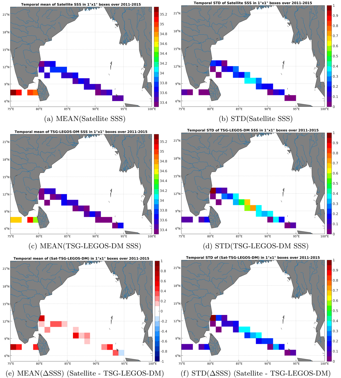
Figure 6: Temporal mean (left) and STD (right) of SSS from Aquarius-L4-IPRC-V4-WEEKLY (top), TSG-LEGOS-DM (middle), and of \Delta SSS (Satellite - TSG-LEGOS-DM). Only match-up pairs are used to generate these maps.
