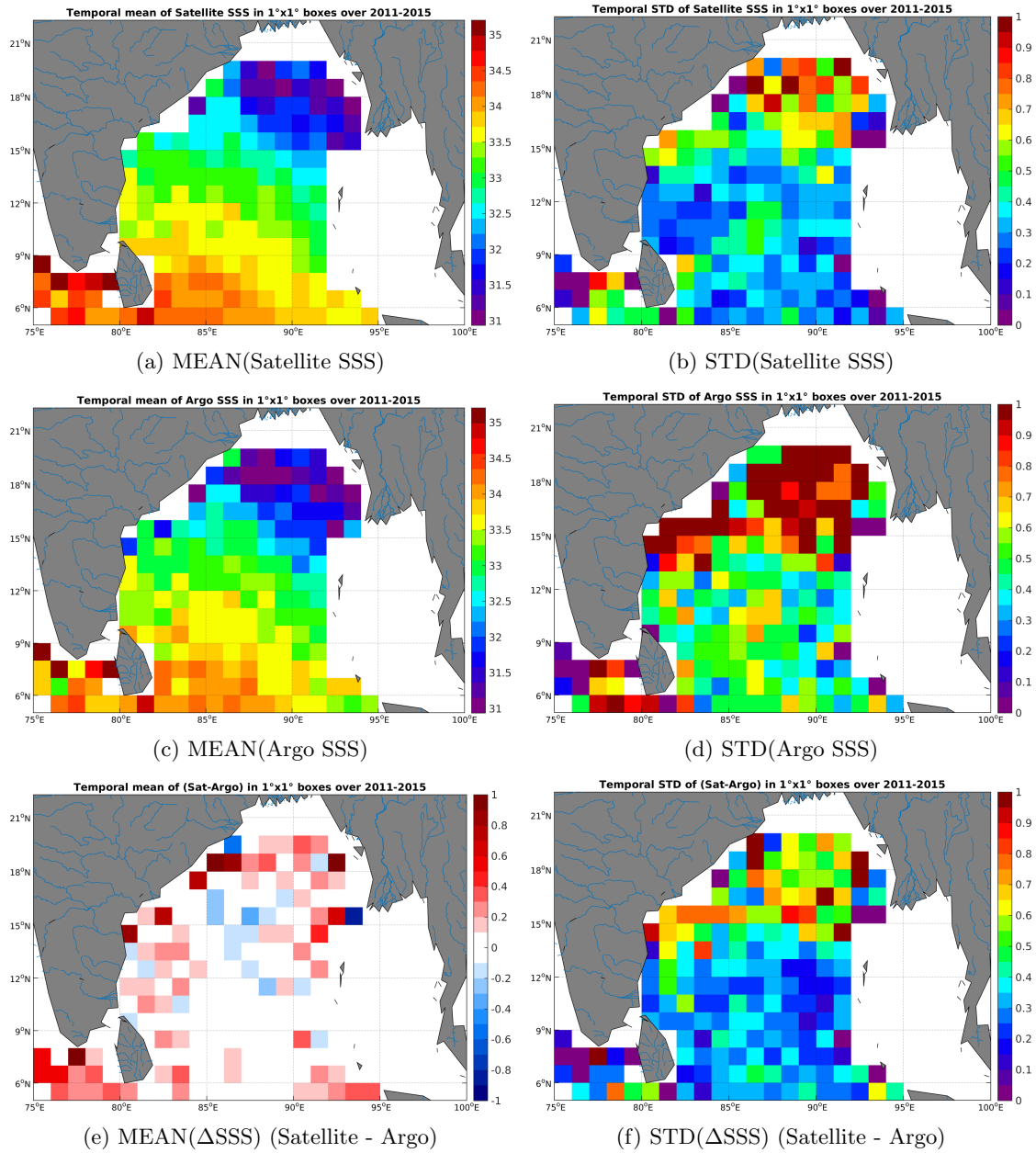
Figure 6: Temporal mean (left) and STD (right) of SSS from Aquarius-L4-IPRC-V4-WEEKLY (top), Argo (middle), and of \Delta SSS (Satellite - Argo). Only match-up pairs are used to generate these maps.
