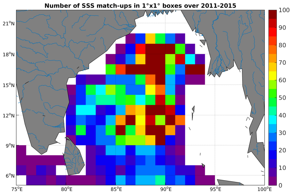
Figure 4: Number of SSS match-ups between Argo SSS and the Aquarius-L4-IPRC-V4-WEEKLY SSS product for the Ganga and Brahmaputra river plumes Pi-MEP region over 1°x1° boxes and for the full satellite product period.
