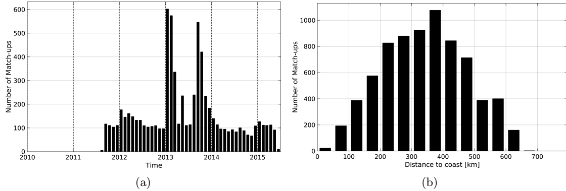
Figure 1: Number of match-ups between Argo and Aquarius-L4-IPRC-V4-WEEKLY SSS as a function of time (a) and as function of the distance to coast (b) over the Ganga and Brahmaputra river plumes Pi-MEP region and for the full satellite product period.
