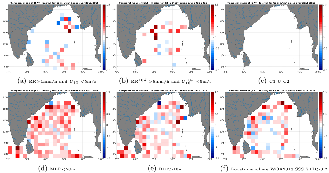
Figure 12: Temporal mean gridded over spatial boxes of size 1^\circ \times 1^\circ of \Delta SSS (Aquarius-L4-IPRC-V4-WEEKLY - Argo) for 6 different subdatasets corresponding to: RR > 1\text{mm/h} and U_{10} < 5\text{m/s} (a), RR^{10d} > 5\text{mm/h} and U_{10}^{10d} < 5\text{m/s} (b), C1 U C2 (c), MLD < 20\text{m} (d), BLT > 10\text{m} (e), Locations where WOA2013 SSS STD > 0.2 (f).
