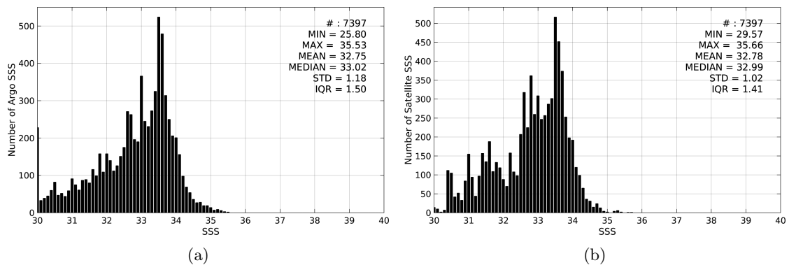
Figure 2: Histograms of SSS from Argo (a) and Aquarius-L4-IPRC-V4-WEEKLY (b) considering all match-up pairs per bins of 0.1 over the Ganga and Brahmaputra river plumes Pi-MEP region and for the full satellite product period.
