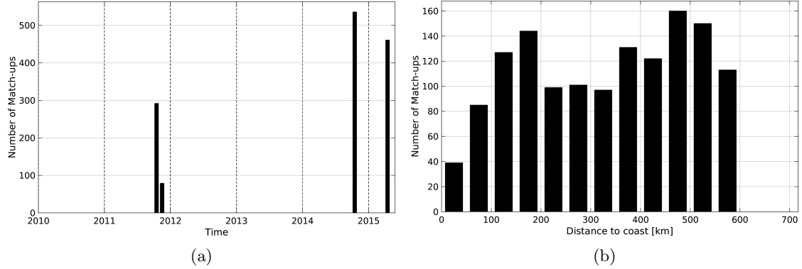
Figure 1: Number of match-ups between TSG-LEGOS-DM and Aquarius-L4-IPRC-V4-MONTHLY SSS as a function of time (a) and as function of the distance to coast (b) over the Ganga and Brahmaputra river plumes Pi-MEP region and for the full satellite product period.
