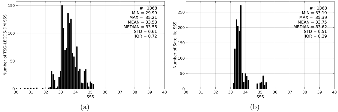
Figure 2: Histograms of SSS from TSG-LEGOS-DM (a) and Aquarius-L4-IPRC-V4-MONTHLY (b) considering all match-up pairs per bins of 0.1 over the Ganga and Brahmaputra river plumes Pi-MEP region and for the full satellite product period.
