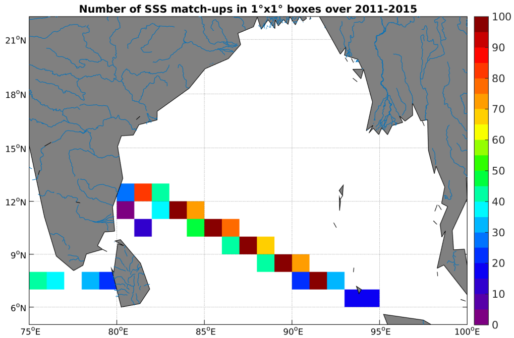
Figure 4: Number of SSS match-ups between TSG-LEGOS-DM SSS and the Aquarius-L4-IPRC-V4-MONTHLY SSS product for the Ganga and Brahmaputra river plumes Pi-MEP region over 1^\circ \times 1^\circ boxes and for the full satellite product period.
