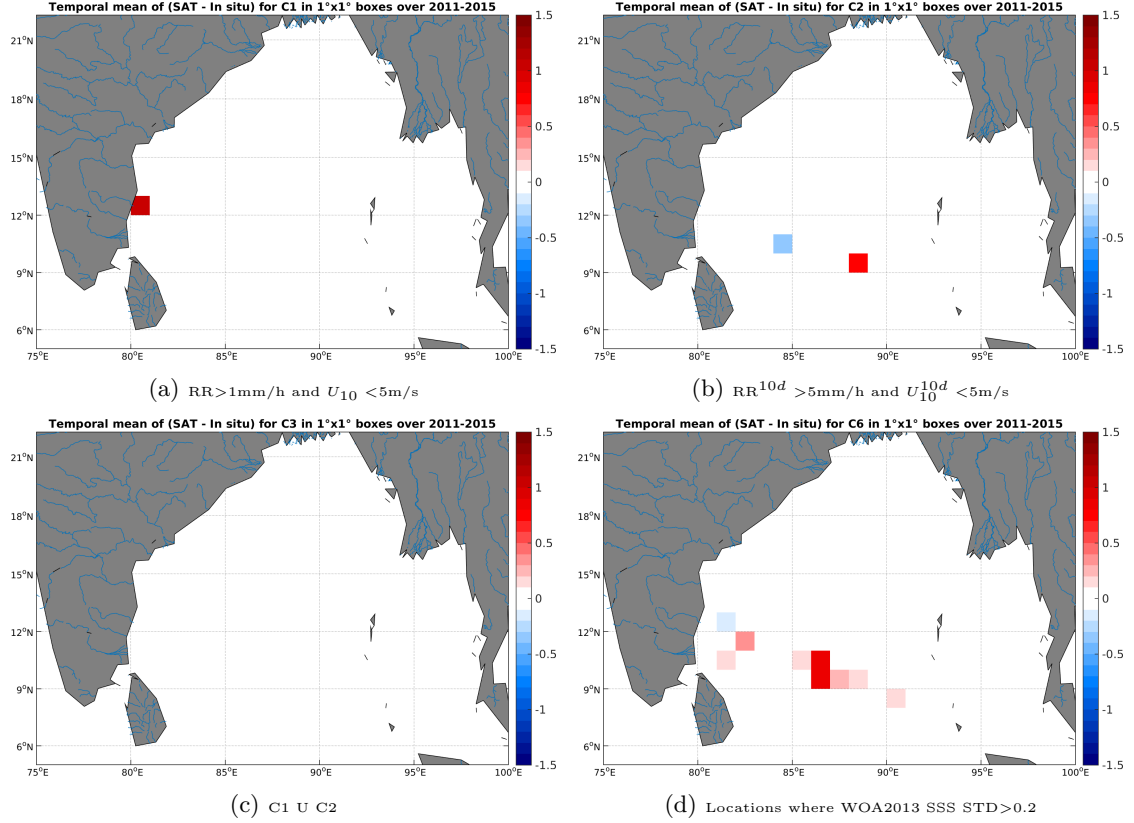
Figure 12: Temporal mean gridded over spatial boxes of size 1^\circ \times 1^\circ of \Delta SSS (Aquarius-L4-IPRC-V4-MONTHLY - TSG-LEGOS-DM) for 4 different subdatasets corresponding to: RR > 1\text{mm/h} and U_{10} < 5\text{m/s} (a), RR^{10d} > 5\text{mm/h} and U_{10}^{10d} < 5\text{m/s} (b), C1 U C2 (c), Locations where WOA2013 SSS STD > 0.2 (d).
