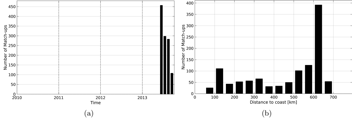
Figure 1: Number of match-ups between Surface drifters and Aquarius-L4-IPRC-V4-MONTHLY SSS as a function of time (a) and as function of the distance to coast (b) over the Ganga and Brahmaputra river plumes Pi-MEP region and for the full satellite product period.
