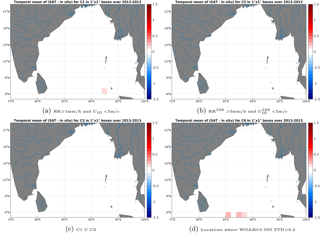
Figure 11: Temporal mean gridded over spatial boxes of size 1^\circ \times 1^\circ of \Delta SSS (Aquarius-L4-IPRC-V4-MONTHLY - Surface drifters) for 4 different subdatasets corresponding to: RR > 1 mm/h and U_{10} < 5 m/s (a), RR 10d > 5 mm/h and U_{10}^{10d} < 5 m/s (b), C1 U C2 (c), Locations where WOA2013 SSS STD > 0.2 (d).
