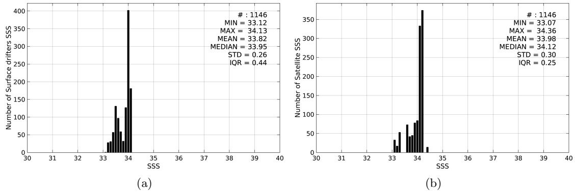
Figure 2: Histograms of SSS from Surface drifters (a) and Aquarius-L4-IPRC-V4-MONTHLY (b) considering all match-up pairs per bins of 0.1 over the Ganga and Brahmaputra river plumes Pi-MEP region and for the full satellite product period.
