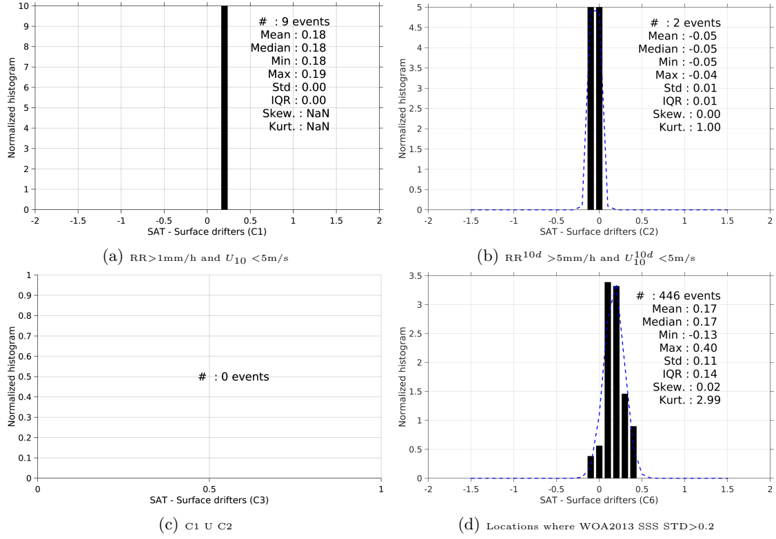
Figure 12: Normalized histogram of \Delta\text{SSS} (Aquarius-L4-IPRC-V4-MONTHLY - Surface drifters) for 6 different subdatasets corresponding to: RR > 1\text{mm/h} and U_{10} < 5\text{m/s} (a), RR^{10d} > 5\text{mm/h} and U_{10}^{10d} < 5\text{m/s} (b), C1 U C2 (c), Locations where WOA2013 SSS STD > 0.2 (d).
