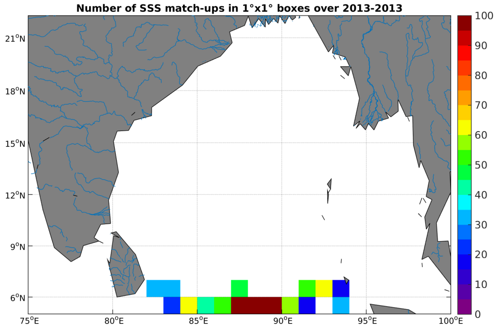
Figure 3: Number of SSS match-ups between Surface drifters SSS and the Aquarius-L4-IPRC-V4-MONTHLY SSS product for the Ganga and Brahmaputra river plumes Pi-MEP region over 1^\circ \times 1^\circ boxes and for the full satellite product period.
