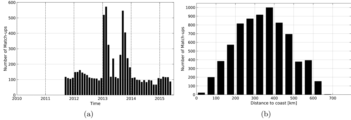
Figure 1: Number of match-ups between Argo and Aquarius-L4-IPRC-V4-MONTHLY SSS as a function of time (a) and as function of the distance to coast (b) over the Ganga and Brahmaputra river plumes Pi-MEP region and for the full satellite product period.
