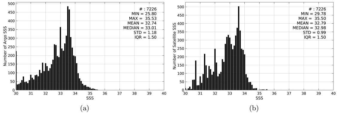
Figure 2: Histograms of SSS from Argo (a) and Aquarius-L4-IPRC-V4-MONTHLY (b) considering all match-up pairs per bins of 0.1 over the Ganga and Brahmaputra river plumes Pi-MEP region and for the full satellite product period.
