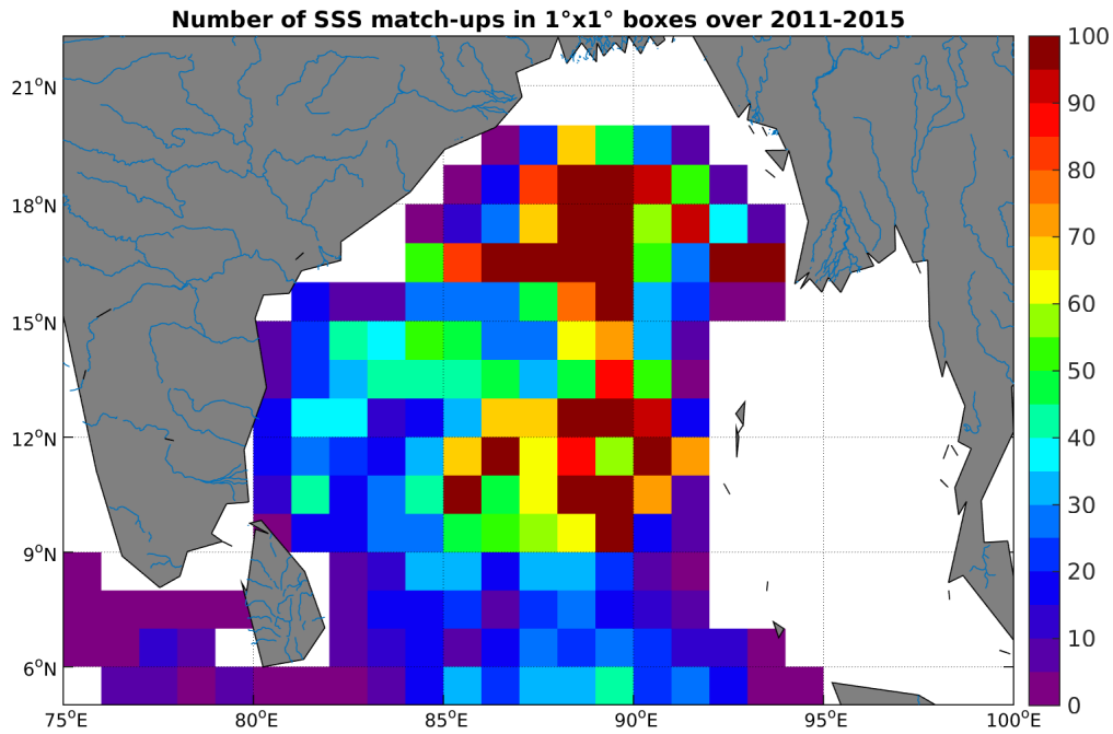
Figure 4: Number of SSS match-ups between Argo SSS and the Aquarius-L4-IPRC-V4-MONTHLY SSS product for the Ganga and Brahmaputra river plumes Pi-MEP region over 1°x1° boxes and for the full satellite product period.
