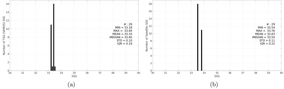
Figure 3: Histograms of SSS from TSG (SAMOS) (a) and Aquarius SSS L3 OR v5 - 7-Day running (NASA-GSFC) (b) considering all match-up pairs per bins of 0.1 over the Ganga and Brahmaputra river plumes Pi-MEP region and for the full satellite product period.
