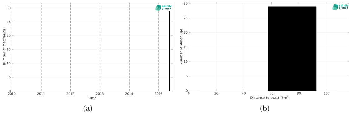
Figure 2: Number of match-ups between TSG (SAMOS) and Aquarius SSS L3 OR v5 - 7-Day running (NASA-GSFC) SSS as a function of time (a) and as function of the distance to coast (b) over the Ganga and Brahmaputra river plumes Pi-MEP region and for the full satellite product period.
