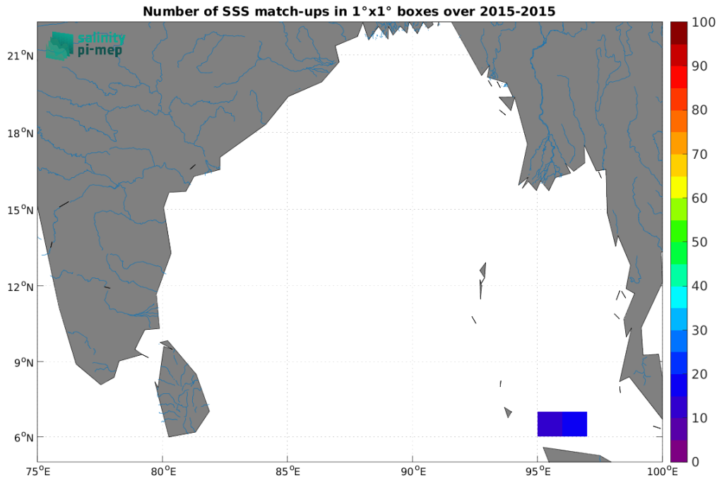
Figure 5: Number of SSS match-ups between TSG (SAMOS) SSS and the Aquarius SSS L3 OR v5 - 7-Day running (NASA-GSFC) SSS product for the Ganga and Brahmaputra river plumes Pi-MEP region over 1^\circ \times 1^\circ boxes and for the full satellite product period.
