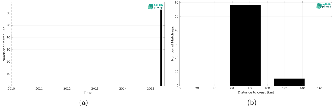
Figure 1: Number of match-ups between TSG (SAMOS) and Aquarius SSS L3 OR v5 - 7-Day running (NASA-GSFC) SSS as a function of time (a) and as function of the distance to coast (b) over the Ganga and Brahmaputra river plumes Pi-MEP region and for the full satellite product period.
