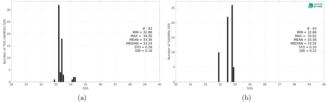
Figure 2: Histograms of SSS from TSG (SAMOS) (a) and Aquarius SSS L3 OR v5 - 7-Day running (NASA-GSFC) (b) considering all match-up pairs per bins of 0.1 over the Ganga and Brahmaputra river plumes Pi-MEP region and for the full satellite product period.
