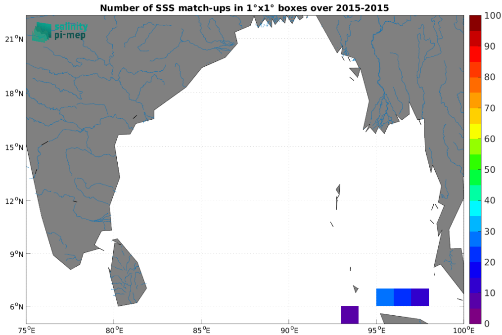
Figure 4: Number of SSS match-ups between TSG (SAMOS) SSS and the Aquarius SSS L3 OR v5 - 7-Day running (NASA-GSFC) SSS product for the Ganga and Brahmaputra river plumes Pi-MEP region over 1^\circ \times 1^\circ boxes and for the full satellite product period.
