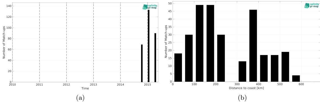
Figure 2: Number of match-ups between TSG (LEGOS-DM) and Aquarius SSS L3 OR v5 - 7-Day running (NASA-GSFC) SSS as a function of time (a) and as function of the distance to coast (b) over the Ganga and Brahmaputra river plumes Pi-MEP region and for the full satellite product period.
