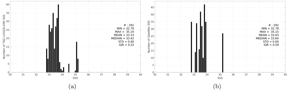
Figure 3: Histograms of SSS from TSG (LEGOS-DM) (a) and Aquarius SSS L3 OR v5 - 7-Day running (NASA-GSFC) (b) considering all match-up pairs per bins of 0.1 over the Ganga and Brahmaputra river plumes Pi-MEP region and for the full satellite product period.
