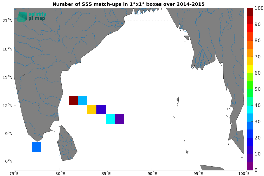
Figure 5: Number of SSS match-ups between TSG (LEGOS-DM) SSS and the Aquarius SSS L3 OR v5 - 7-Day running (NASA-GSFC) SSS product for the Ganga and Brahmaputra river plumes Pi-MEP region over 1^\circ \times 1^\circ boxes and for the full satellite product period.
