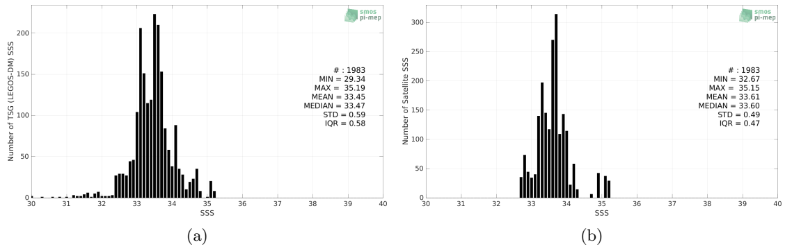
Figure 2: Histograms of SSS from TSG (LEGOS-DM) (a) and Aquarius SSS L3 OR v5 - 7-Day running (NASA-GSFC) (b) considering all match-up pairs per bins of 0.1 over the Ganga and Brahmaputra river plumes Pi-MEP region and for the full satellite product period.
