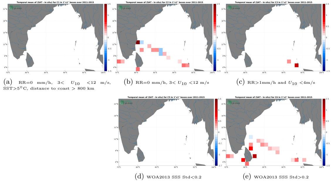
Figure 12: Temporal mean gridded over spatial boxes of size 1^{\circ}\times 1^{\circ} of \Delta\text{SSS} (Aquarius SSS L3 OR v5 - 7-Day running (NASA-GSFC) - TSG (LEGOS-DM)) for 5 different subdatasets corresponding to:RR=0 mm/h, 3 < U_{10} < 12 m/s, SST >5^{\circ}\text{C} , distance to coast > 800 km (a), RR=0 mm/h, 3 < U_{10} < 12 m/s (b), RR >1 mm/h and U_{10} < 4 m/s (c), WOA2013 SSS Std <0.2 (d), WOA2013 SSS Std >0.2 (e).
