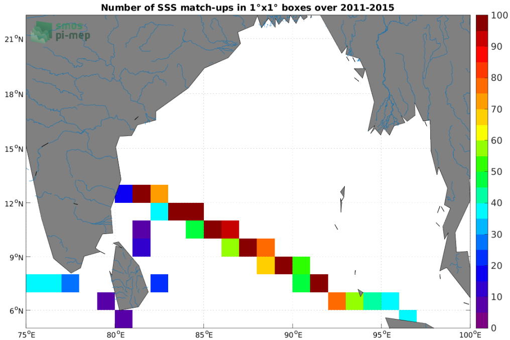
Figure 4: Number of SSS match-ups between TSG (LEGOS-DM) SSS and the Aquarius SSS L3 OR v5 - 7-Day running (NASA-GSFC) SSS product for the Ganga and Brahmaputra river plumes Pi-MEP region over 1^\circ \times 1^\circ boxes and for the full satellite product period.
