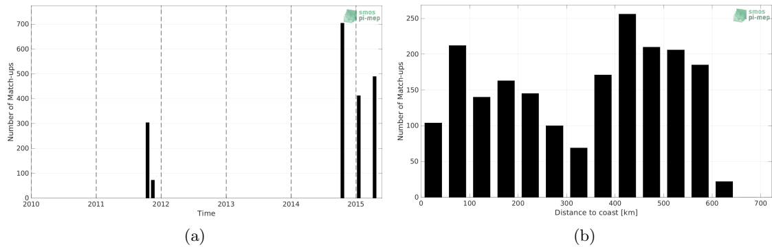
Figure 1: Number of match-ups between TSG (LEGOS-DM) and Aquarius SSS L3 OR v5 - 7-Day running (NASA-GSFC) SSS as a function of time (a) and as function of the distance to coast (b) over the Ganga and Brahmaputra river plumes Pi-MEP region and for the full satellite product period.
