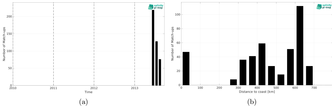
Figure 2: Number of match-ups between Surface drifters and Aquarius SSS L3 OR v5 - 7-Day running (NASA-GSFC) SSS as a function of time (a) and as function of the distance to coast (b) over the Ganga and Brahmaputra river plumes Pi-MEP region and for the full satellite product period.
