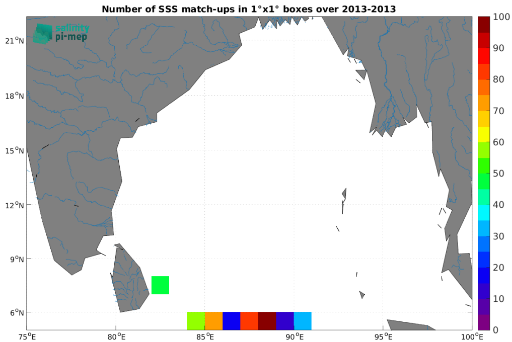
Figure 4: Number of SSS match-ups between Surface drifters SSS and the Aquarius SSS L3 OR v5 - 7-Day running (NASA-GSFC) SSS product for the Ganga and Brahmaputra river plumes Pi-MEP region over 1°x1° boxes and for the full satellite product period.
