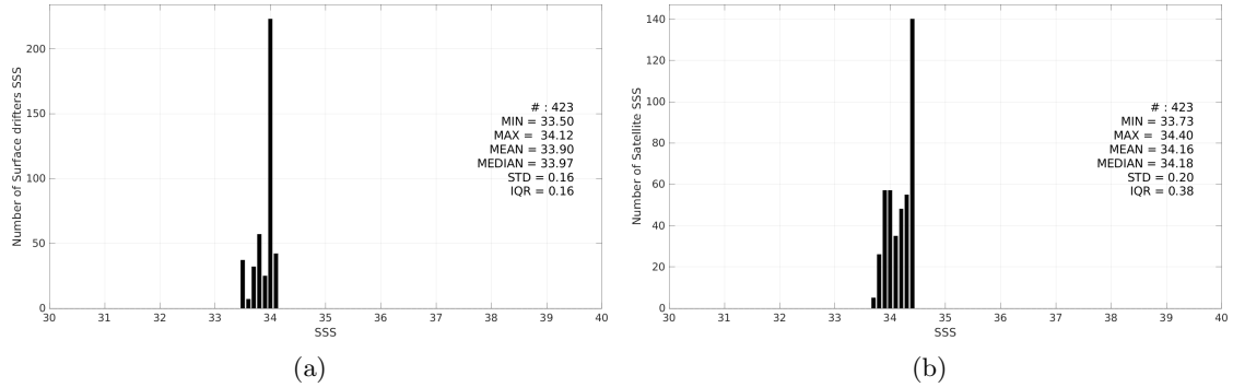
Figure 3: Histograms of SSS from Surface drifters (a) and Aquarius SSS L3 OR v5 - 7-Day running (NASA-GSFC) (b) considering all match-up pairs per bins of 0.1 over the Ganga and Brahmaputra river plumes Pi-MEP region and for the full satellite product period.
