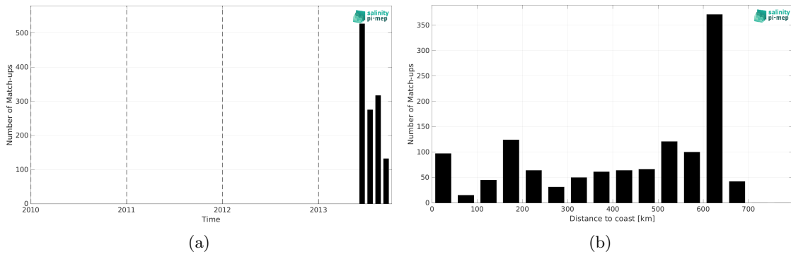
Figure 1: Number of match-ups between Surface drifters and Aquarius SSS L3 OR v5 - 7-Day running (NASA-GSFC) SSS as a function of time (a) and as function of the distance to coast (b) over the Ganga and Brahmaputra river plumes Pi-MEP region and for the full satellite product period.
