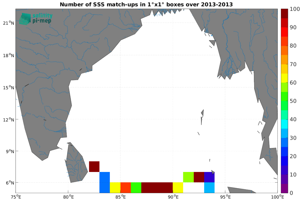
Figure 3: Number of SSS match-ups between Surface drifters SSS and the Aquarius SSS L3 OR v5 - 7-Day running (NASA-GSFC) SSS product for the Ganga and Brahmaputra river plumes Pi-MEP region over 1°x1° boxes and for the full satellite product period.
