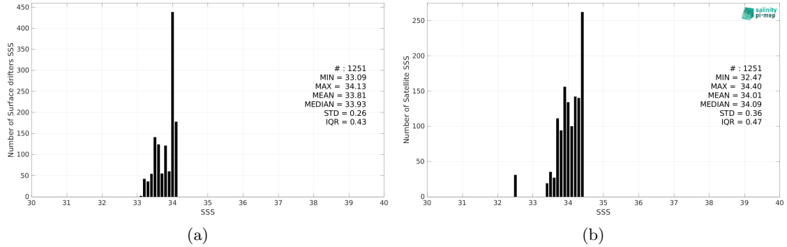
Figure 2: Histograms of SSS from Surface drifters (a) and Aquarius SSS L3 OR v5 - 7-Day running (NASA-GSFC) (b) considering all match-up pairs per bins of 0.1 over the Ganga and Brahmaputra river plumes Pi-MEP region and for the full satellite product period.
