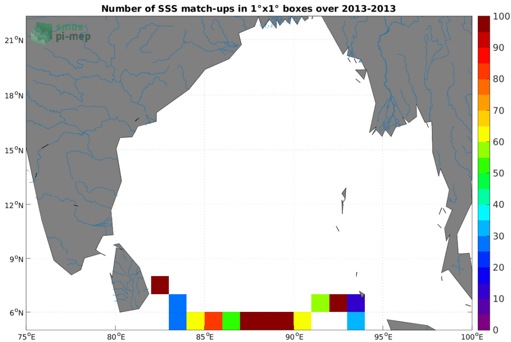
Figure 3: Number of SSS match-ups between Surface drifters SSS and the Aquarius SSS L3 OR v5 - 7-Day running (NASA-GSFC) SSS product for the Ganga and Brahmaputra river plumes Pi-MEP region over 1^\circ \times 1^\circ boxes and for the full satellite product period.
