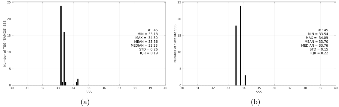
Figure 3: Histograms of SSS from TSG (SAMOS) (a) and Aquarius SSS L3 OR v5 - 7-Day running - Rain mask (NASA-GSFC) (b) considering all match-up pairs per bins of 0.1 over the Ganga and Brahmaputra river plumes Pi-MEP region and for the full satellite product period.
