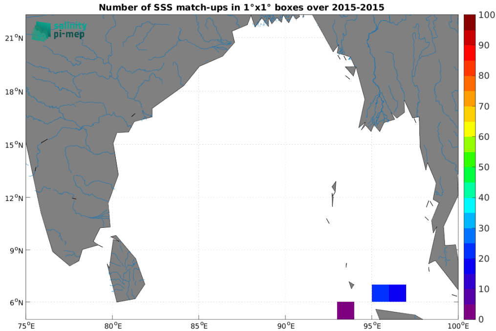
Figure 5: Number of SSS match-ups between TSG (SAMOS) SSS and the Aquarius SSS L3 OR v5 - 7-Day running - Rain mask (NASA-GSFC) SSS product for the Ganga and Brahmaputra river plumes Pi-MEP region over 1^\circ \times 1^\circ boxes and for the full satellite product period.
