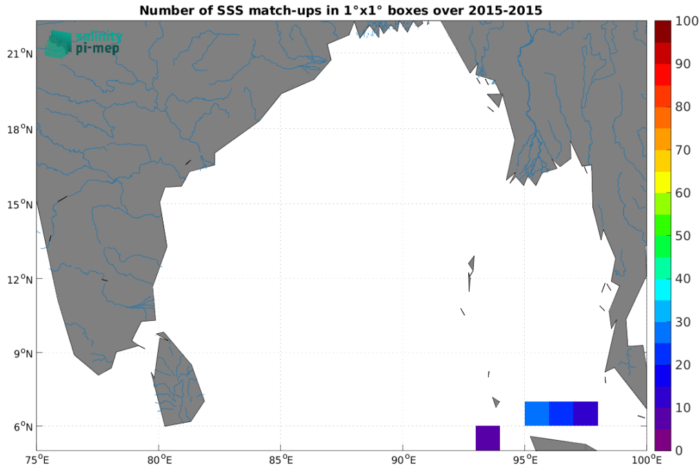
Figure 4: Number of SSS match-ups between TSG (SAMOS) SSS and the Aquarius SSS L3 OR v5 - 7-Day running - Rain mask (NASA-GSFC) SSS product for the Ganga and Brahmaputra river plumes Pi-MEP region over 1^\circ \times 1^\circ boxes and for the full satellite product period.
