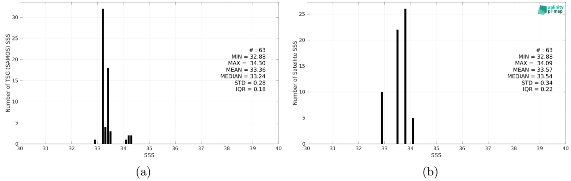
Figure 2: Histograms of SSS from TSG (SAMOS) (a) and Aquarius SSS L3 OR v5 - 7-Day running - Rain mask (NASA-GSFC) (b) considering all match-up pairs per bins of 0.1 over the Ganga and Brahmaputra river plumes Pi-MEP region and for the full satellite product period.
