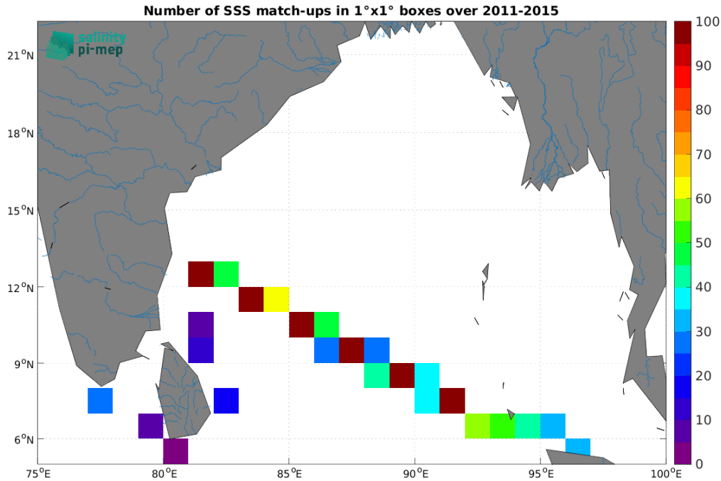
Figure 5: Number of SSS match-ups between TSG (LEGOS-DM) SSS and the Aquarius SSS L3 OR v5 - 7-Day running - Rain mask (NASA-GSFC) SSS product for the Ganga and Brahmaputra river plumes Pi-MEP region over 1^\circ \times 1^\circ boxes and for the full satellite product period.
