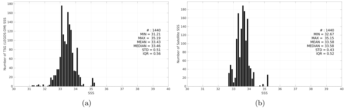
Figure 3: Histograms of SSS from TSG (LEGOS-DM) (a) and Aquarius SSS L3 OR v5 - 7-Day running - Rain mask (NASA-GSFC) (b) considering all match-up pairs per bins of 0.1 over the Ganga and Brahmaputra river plumes Pi-MEP region and for the full satellite product period.
