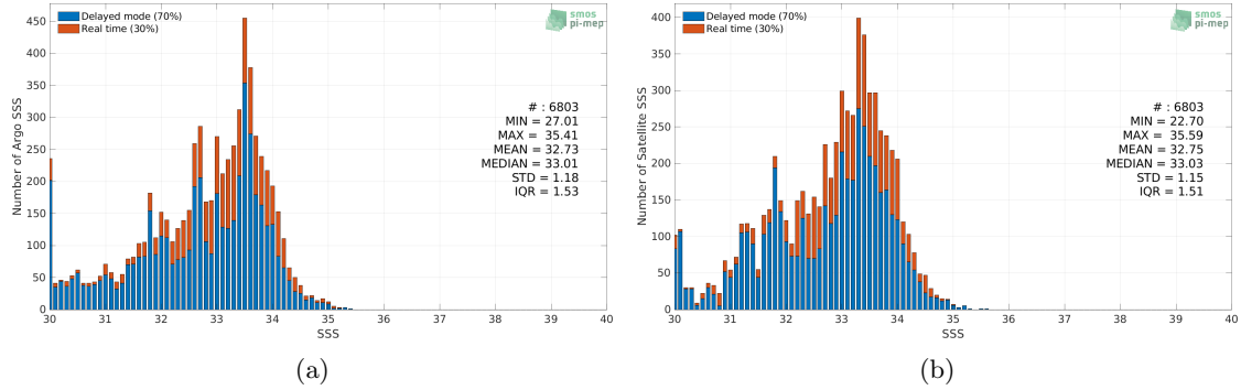
Figure 2: Histograms of SSS from Argo (a) and Aquarius SSS L3 OR v5 - 7-Day running - Rain mask (NASA-GSFC) (b) considering all match-up pairs per bins of 0.1 over the Ganga and Brahmaputra river plumes Pi-MEP region and for the full satellite product period.
