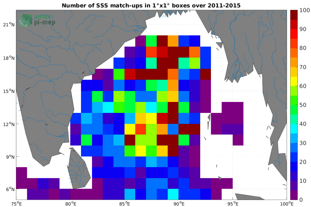
Figure 4: Number of SSS match-ups between Argo SSS and the Aquarius SSS L3 OR v5 - 7-Day running - Rain mask (NASA-GSFC) SSS product for the Ganga and Brahmaputra river plumes Pi-MEP region over 1^\circ \times 1^\circ boxes and for the full satellite product period.
