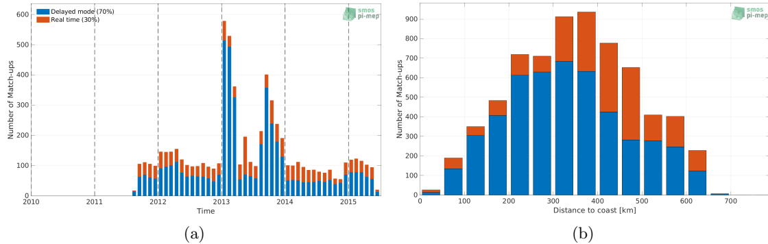
Figure 1: Number of match-ups between Argo and Aquarius SSS L3 OR v5 - 7-Day running - Rain mask (NASA-GSFC) SSS as a function of time (a) and as function of the distance to coast (b) over the Ganga and Brahmaputra river plumes Pi-MEP region and for the full satellite product period.
