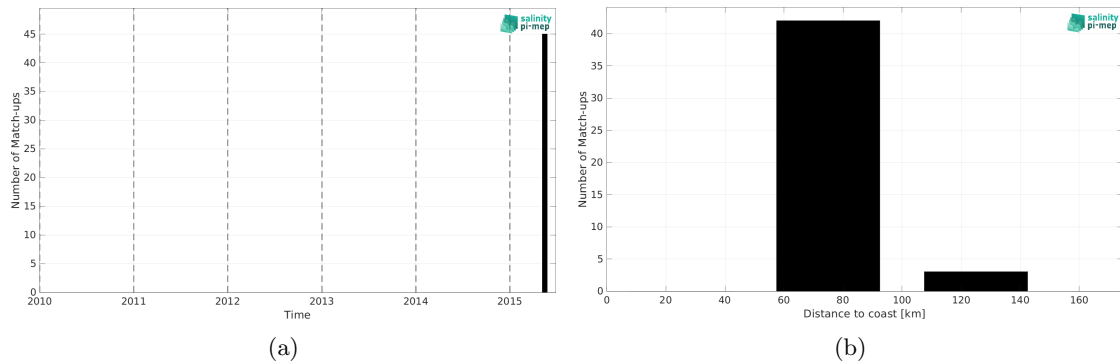
Figure 2: Number of match-ups between TSG (SAMOS) and Aquarius SSS L3 OR v5 - Monthly (NASA-GSFC) SSS as a function of time (a) and as function of the distance to coast (b) over the Ganga and Brahmaputra river plumes Pi-MEP region and for the full satellite product period.
