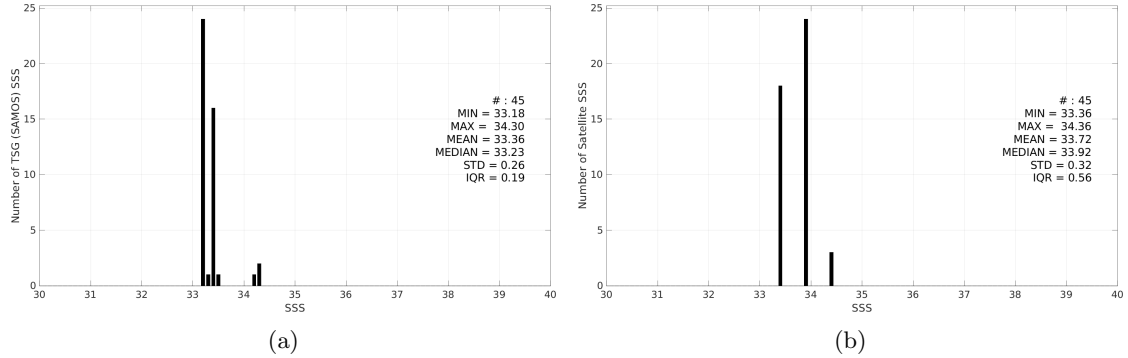
Figure 3: Histograms of SSS from TSG (SAMOS) (a) and Aquarius SSS L3 OR v5 - Monthly (NASA-GSFC) (b) considering all match-up pairs per bins of 0.1 over the Ganga and Brahmaputra river plumes Pi-MEP region and for the full satellite product period.
