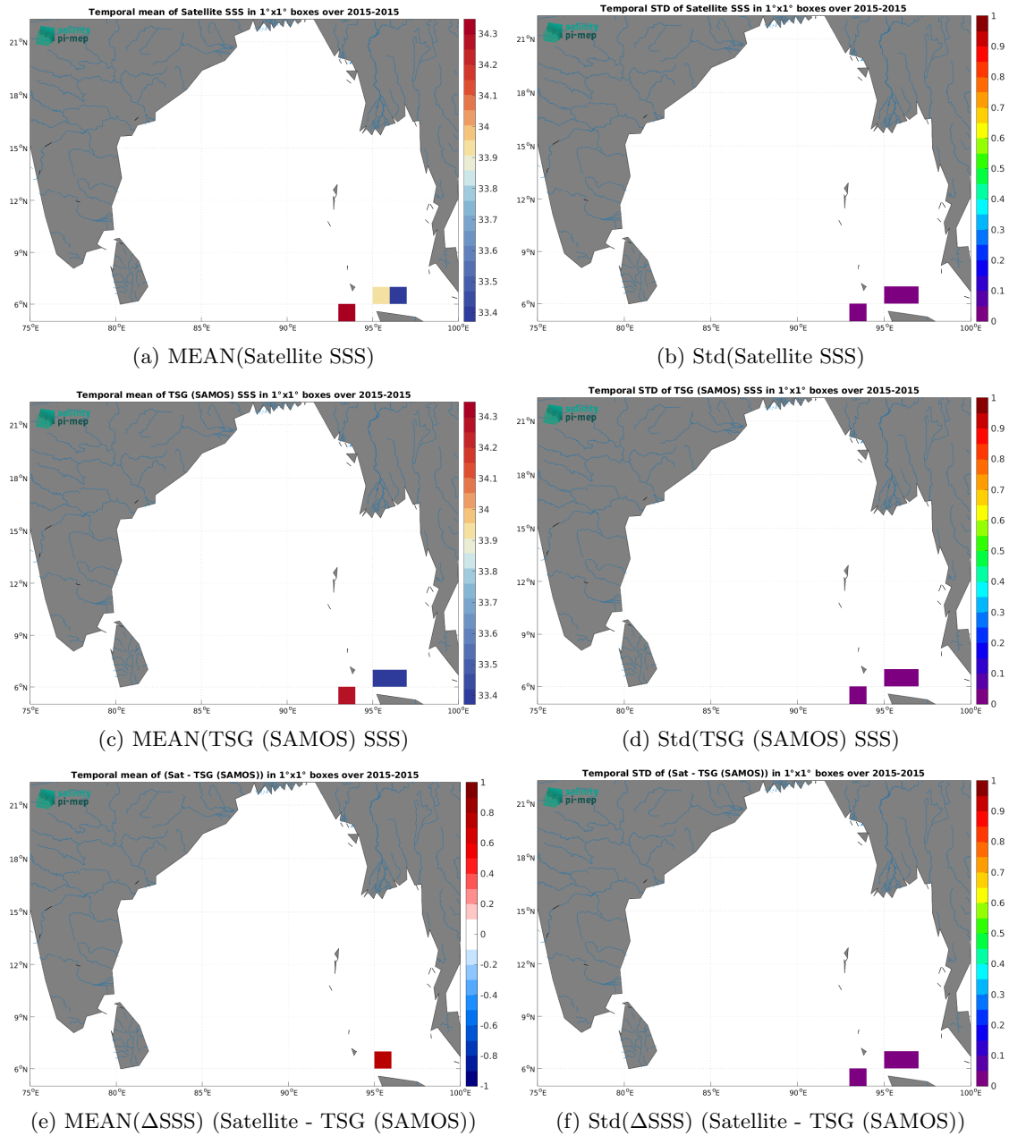
Figure 7: Temporal mean (left) and Std (right) of SSS from Aquarius SSS L3 OR v5 - Monthly (NASA-GSFC) (top), TSG (SAMOS) (middle), and of \Delta SSS (Satellite - TSG (SAMOS)). Only match-up pairs are used to generate these maps.
