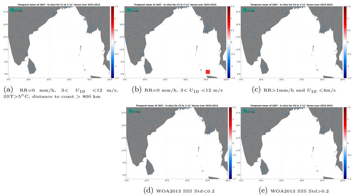
Figure 14: Temporal mean gridded over spatial boxes of size 1^\circ \times 1^\circ of \Delta SSS (Aquarius SSS L3 OR v5 - Monthly (NASA-GSFC) - TSG (SAMOS)) for 5 different subdatasets corresponding to:RR=0 mm/h, 3 < U_{10} < 12 m/s, SST >5^\circ C, distance to coast > 800 km (a), RR=0 mm/h, 3 < U_{10} < 12 m/s (b), RR >1 mm/h and U_{10} < 4 m/s (c), WOA2013 SSS Std <0.2 (d), WOA2013 SSS Std >0.2 (e).
