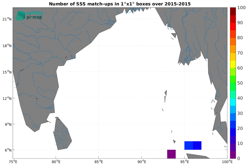
Figure 5: Number of SSS match-ups between TSG (SAMOS) SSS and the Aquarius SSS L3 OR v5 - Monthly (NASA-GSFC) SSS product for the Ganga and Brahmaputra river plumes Pi-MEP region over 1^\circ \times 1^\circ boxes and for the full satellite product period.
