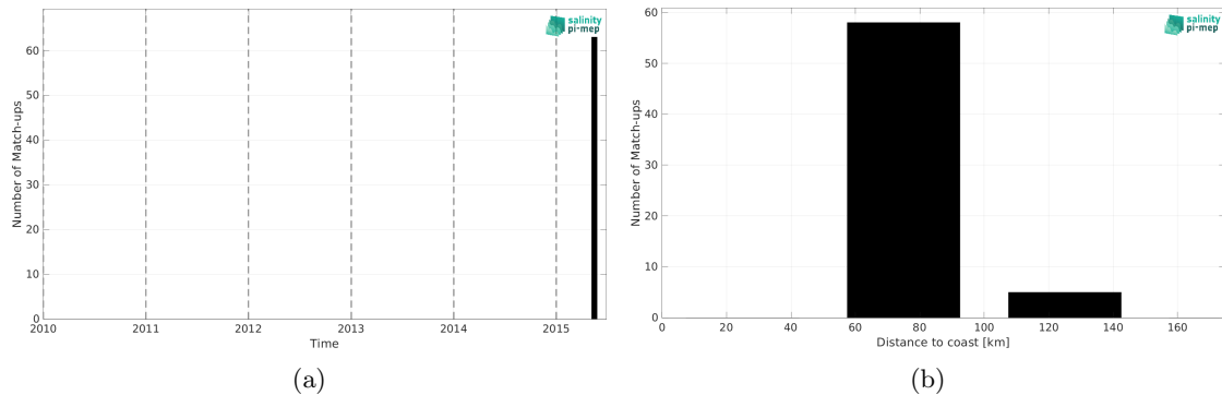
Figure 1: Number of match-ups between TSG (SAMOS) and Aquarius SSS L3 OR v5 - Monthly (NASA-GSFC) SSS as a function of time (a) and as function of the distance to coast (b) over the Ganga and Brahmaputra river plumes Pi-MEP region and for the full satellite product period.
