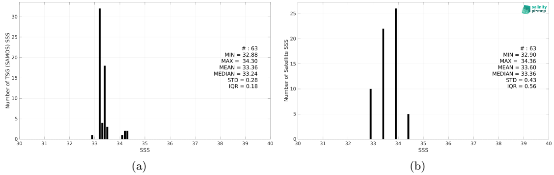
Figure 2: Histograms of SSS from TSG (SAMOS) (a) and Aquarius SSS L3 OR v5 - Monthly (NASA-GSFC) (b) considering all match-up pairs per bins of 0.1 over the Ganga and Brahmaputra river plumes Pi-MEP region and for the full satellite product period.
