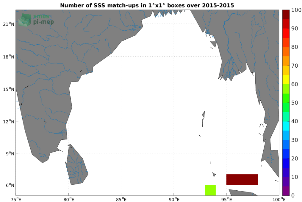
Figure 4: Number of SSS match-ups between TSG (SAMOS) SSS and the Aquarius SSS L3 OR v5 - Monthly (NASA-GSFC) SSS product for the Ganga and Brahmaputra river plumes Pi-MEP region over 1^{\circ} \times 1^{\circ} boxes and for the full satellite product period.
