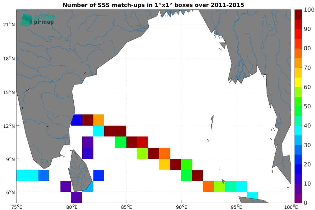
Figure 4: Number of SSS match-ups between TSG (LEGOS-DM) SSS and the Aquarius SSS L3 OR v5 - Monthly (NASA-GSFC) SSS product for the Ganga and Brahmaputra river plumes Pi-MEP region over 1^\circ \times 1^\circ boxes and for the full satellite product period.
