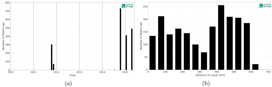
Figure 1: Number of match-ups between TSG (LEGOS-DM) and Aquarius SSS L3 OR v5 - Monthly (NASA-GSFC) SSS as a function of time (a) and as function of the distance to coast (b) over the Ganga and Brahmaputra river plumes Pi-MEP region and for the full satellite product period.
