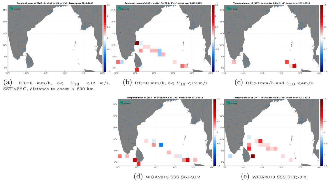
Figure 12: Temporal mean gridded over spatial boxes of size 1^{\circ}\times 1^{\circ} of \Delta\text{SSS} (Aquarius SSS L3 OR v5 - Monthly (NASA-GSFC) - TSG (LEGOS-DM)) for 5 different subdatasets corresponding to:RR=0 mm/h, 3 < U_{10} < 12 m/s, SST >5^{\circ}\text{C} , distance to coast > 800 km (a), RR=0 mm/h, 3 < U_{10} < 12 m/s (b), RR >1 mm/h and U_{10} < 4 m/s (c), WOA2013 SSS Std <0.2 (d), WOA2013 SSS Std >0.2 (e).
