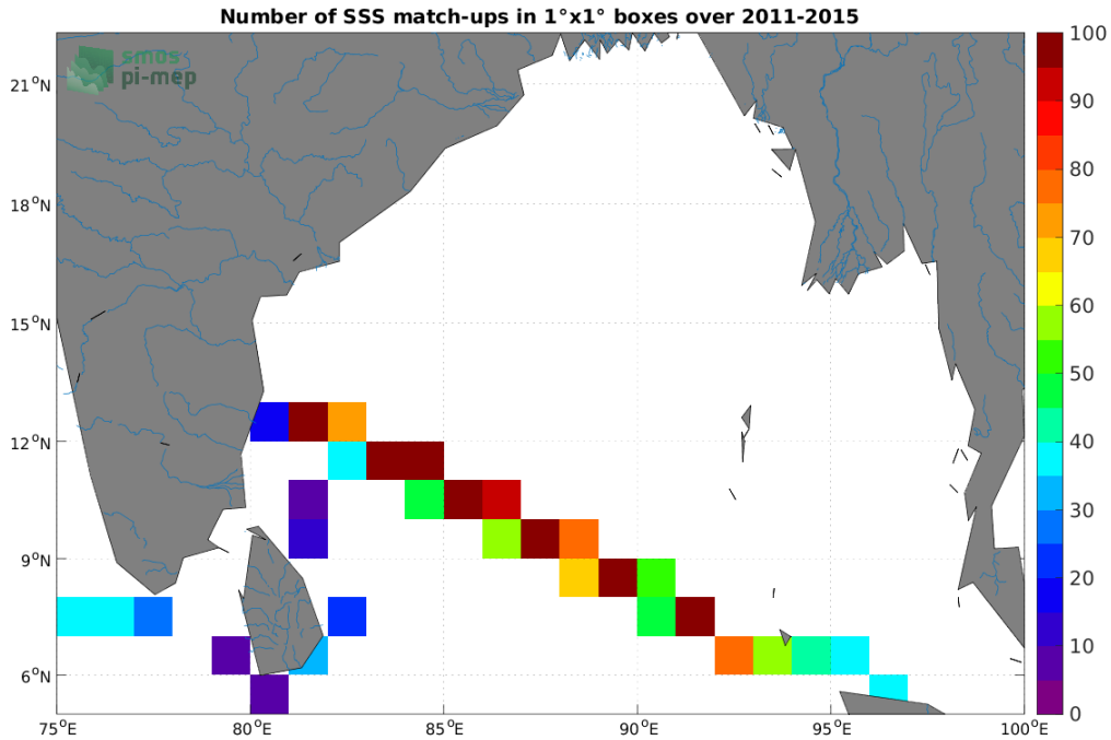
Figure 4: Number of SSS match-ups between TSG (LEGOS-DM) SSS and the Aquarius SSS L3 OR v5 - Monthly (NASA-GSFC) SSS product for the Ganga and Brahmaputra river plumes Pi-MEP region over 1^{\circ} \times 1^{\circ} boxes and for the full satellite product period.
