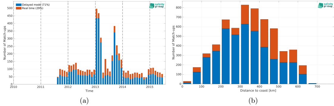
Figure 2: Number of match-ups between Argo and Aquarius SSS L3 OR v5 - Monthly (NASA-GSFC) SSS as a function of time (a) and as function of the distance to coast (b) over the Ganga and Brahmaputra river plumes Pi-MEP region and for the full satellite product period.
