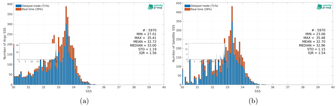
Figure 3: Histograms of SSS from Argo (a) and Aquarius SSS L3 OR v5 - Monthly (NASA-GSFC) (b) considering all match-up pairs per bins of 0.1 over the Ganga and Brahmaputra river plumes Pi-MEP region and for the full satellite product period.
