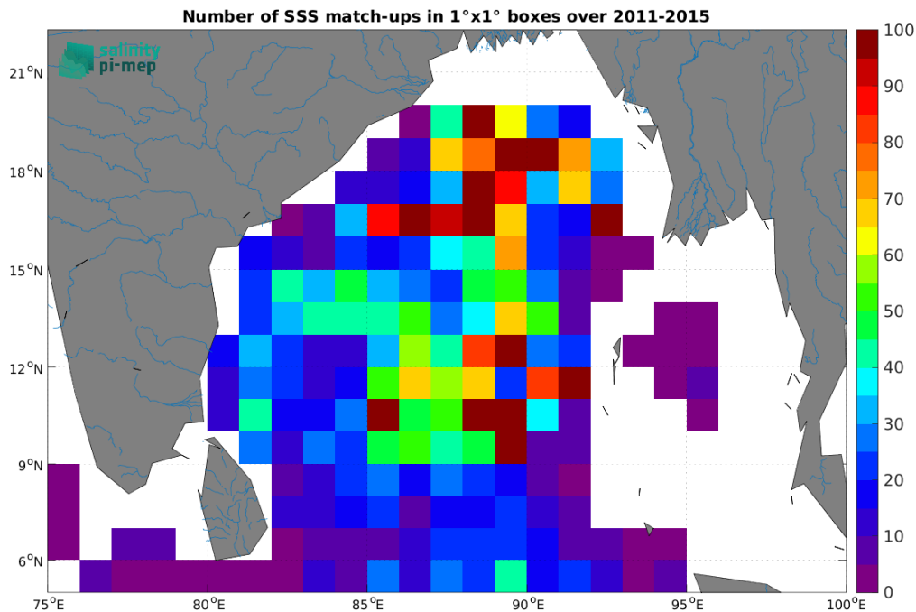
Figure 5: Number of SSS match-ups between Argo SSS and the Aquarius SSS L3 OR v5 - Monthly (NASA-GSFC) SSS product for the Ganga and Brahmaputra river plumes Pi-MEP region over 1^\circ \times 1^\circ boxes and for the full satellite product period.
