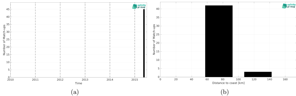
Figure 2: Number of match-ups between TSG (SAMOS) and Aquarius SSS L3 OR v5 - Monthly - Rain mask (NASA-GSFC) SSS as a function of time (a) and as function of the distance to coast (b) over the Ganga and Brahmaputra river plumes Pi-MEP region and for the full satellite product period.
