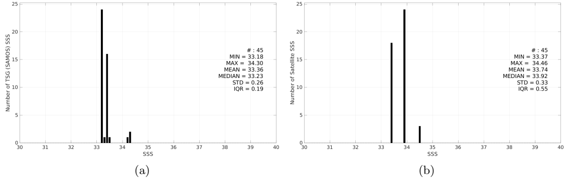
Figure 3: Histograms of SSS from TSG (SAMOS) (a) and Aquarius SSS L3 OR v5 - Monthly - Rain mask (NASA-GSFC) (b) considering all match-up pairs per bins of 0.1 over the Ganga and Brahmaputra river plumes Pi-MEP region and for the full satellite product period.
