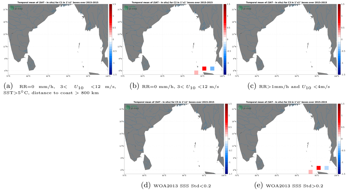
Figure 12: Temporal mean gridded over spatial boxes of size 1^{\circ}\times 1^{\circ} of \Delta\text{SSS} (Aquarius SSS L3 OR v5 - Monthly - Rain mask (NASA-GSFC) - TSG (SAMOS)) for 5 different subdatasets corresponding to:RR=0 mm/h, 3 < U_{10} < 12 m/s, SST >5^{\circ}\text{C} , distance to coast > 800 km (a), RR=0 mm/h, 3 < U_{10} < 12 m/s (b), RR >1 mm/h and U_{10} < 4 m/s (c), WOA2013 SSS Std <0.2 (d), WOA2013 SSS Std >0.2 (e).
