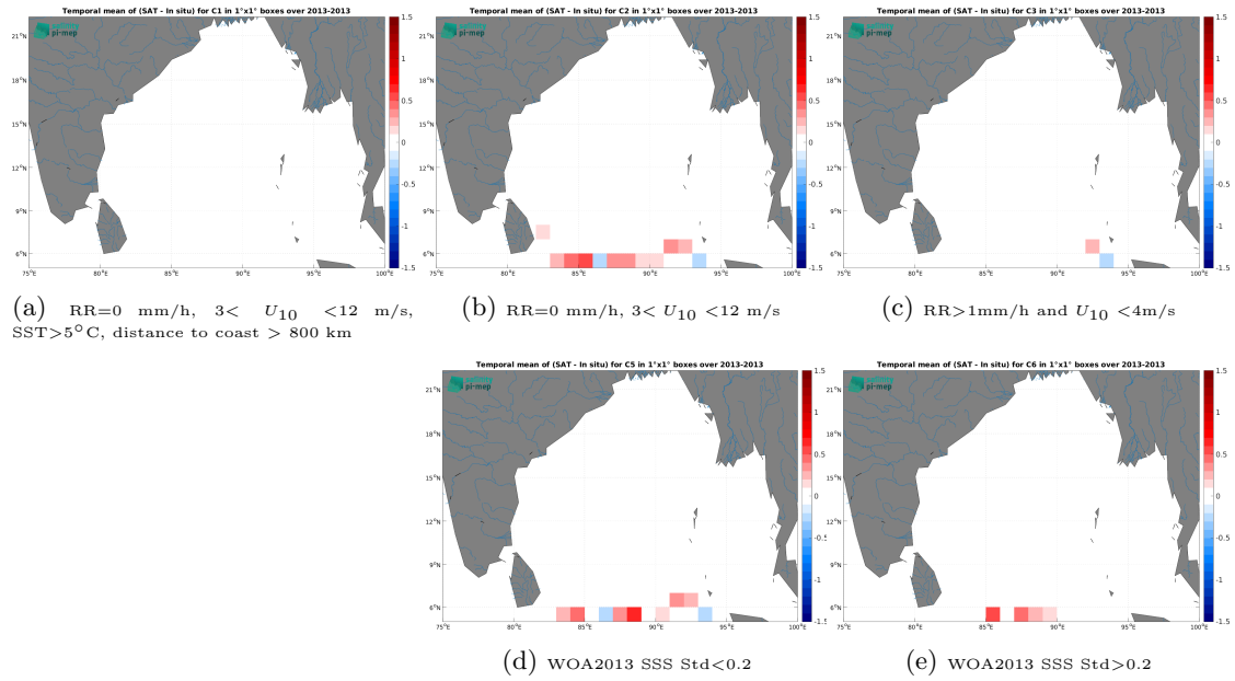
Figure 13: Temporal mean gridded over spatial boxes of size 1^\circ \times 1^\circ of \Delta SSS (Aquarius SSS L3 OR v5 - Monthly - Rain mask (NASA-GSFC) - Surface drifters) for 5 different subdatasets corresponding to:RR=0 mm/h, 3 < U_{10} < 12 m/s, SST >5^\circ\text{C} , distance to coast > 800 km (a), RR=0 mm/h, 3 < U_{10} < 12 m/s (b), RR >1 mm/h and U_{10} < 4 m/s (c), WOA2013 SSS Std <0.2 (d), WOA2013 SSS Std >0.2 (e).
