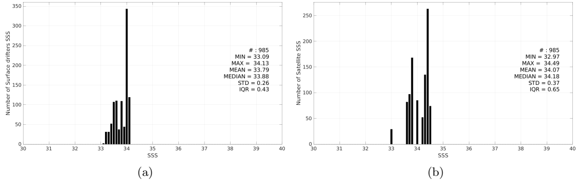
Figure 3: Histograms of SSS from Surface drifters (a) and Aquarius SSS L3 OR v5 - Monthly - Rain mask (NASA-GSFC) (b) considering all match-up pairs per bins of 0.1 over the Ganga and Brahmaputra river plumes Pi-MEP region and for the full satellite product period.
