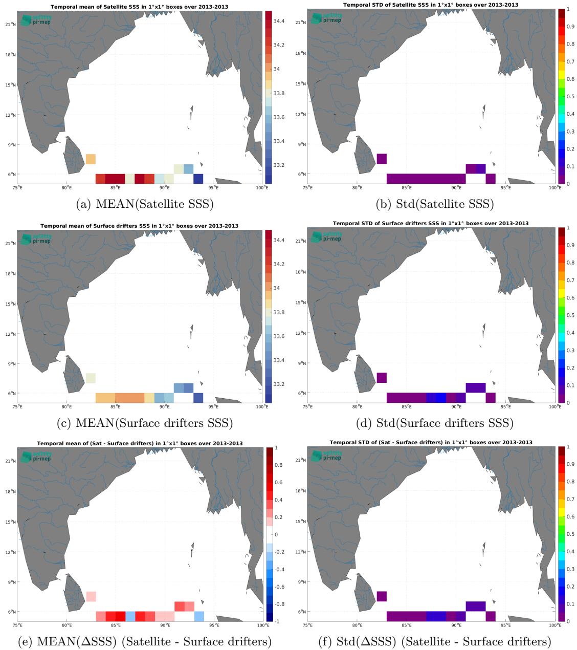
Figure 6: Temporal mean (left) and Std (right) of SSS from Aquarius SSS L3 OR v5 - Monthly - Rain mask (NASA-GSFC) (top), Surface drifters (middle), and of \Delta SSS (Satellite - Surface drifters). Only match-up pairs are used to generate these maps.
