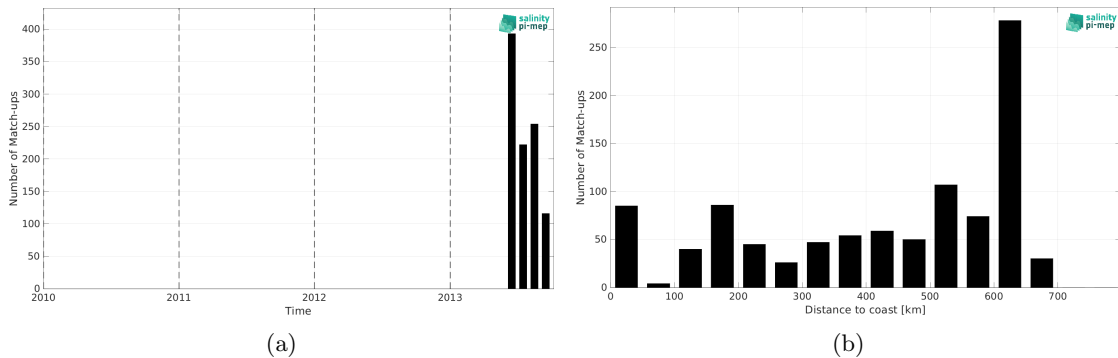
Figure 2: Number of match-ups between Surface drifters and Aquarius SSS L3 OR v5 - Monthly - Rain mask (NASA-GSFC) SSS as a function of time (a) and as function of the distance to coast (b) over the Ganga and Brahmaputra river plumes Pi-MEP region and for the full satellite product period.
