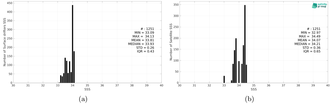
Figure 2: Histograms of SSS from Surface drifters (a) and Aquarius SSS L3 OR v5 - Monthly - Rain mask (NASA-GSFC) (b) considering all match-up pairs per bins of 0.1 over the Ganga and Brahmaputra river plumes Pi-MEP region and for the full satellite product period.
