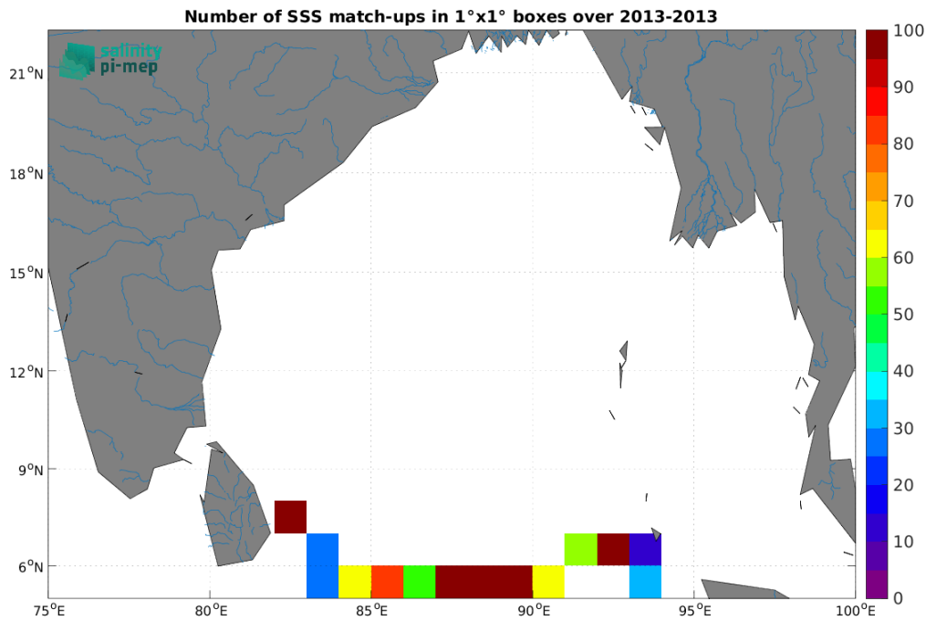
Figure 3: Number of SSS match-ups between Surface drifters SSS and the Aquarius SSS L3 OR v5 - Monthly - Rain mask (NASA-GSFC) SSS product for the Ganga and Brahmaputra river plumes Pi-MEP region over 1^\circ \times 1^\circ boxes and for the full satellite product period.
