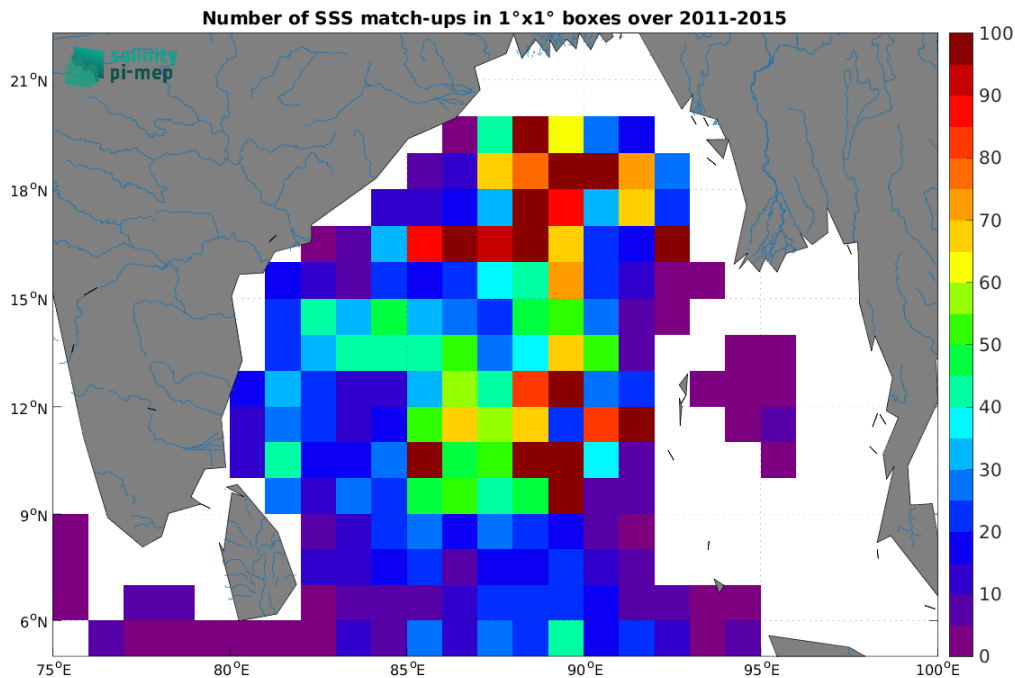
Figure 5: Number of SSS match-ups between Argo SSS and the Aquarius SSS L3 OR v5 - Monthly - Rain mask (NASA-GSFC) SSS product for the Ganga and Brahmaputra river plumes Pi-MEP region over 1^\circ \times 1^\circ boxes and for the full satellite product period.
