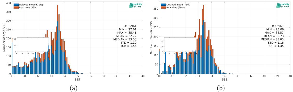
Figure 3: Histograms of SSS from Argo (a) and Aquarius SSS L3 OR v5 - Monthly - Rain mask (NASA-GSFC) (b) considering all match-up pairs per bins of 0.1 over the Ganga and Brahmaputra river plumes Pi-MEP region and for the full satellite product period.
