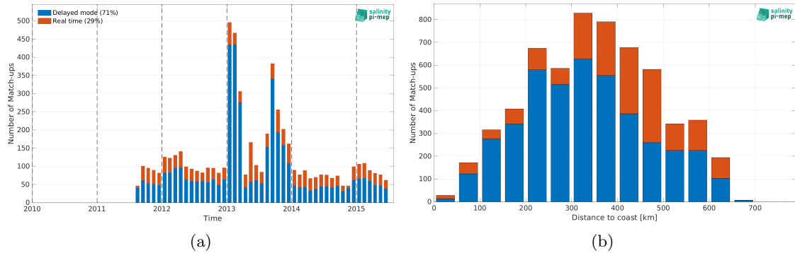
Figure 2: Number of match-ups between Argo and Aquarius SSS L3 OR v5 - Monthly - Rain mask (NASA-GSFC) SSS as a function of time (a) and as function of the distance to coast (b) over the Ganga and Brahmaputra river plumes Pi-MEP region and for the full satellite product period.
