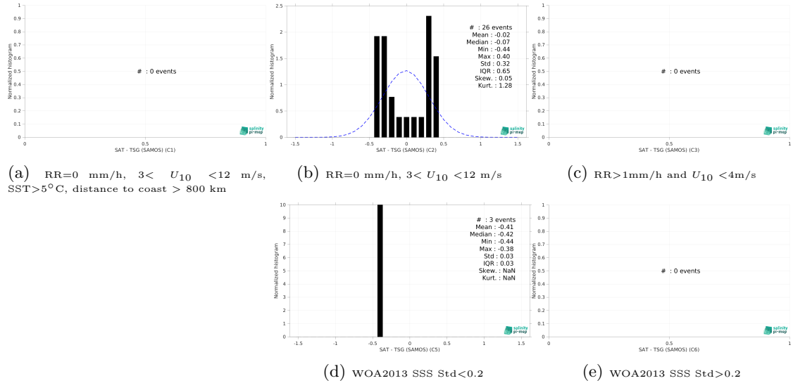
Figure 15: Normalized histogram of \Delta SSS (Aquarius SSS L3 CAP v5 - 7-Day running (JPL) - TSG (SAMOS)) for 5 different subdatasets corresponding to: RR=0 mm/h, 3 < U_{10} < 12 m/s, SST>5°C, distance to coast > 800 km (a), RR=0 mm/h, 3 < U_{10} < 12 m/s (b), RR>1mm/h and U_{10} < 4 m/s (c), WOA2013 SSS Std<0.2 (d), WOA2013 SSS Std>0.2 (e).
