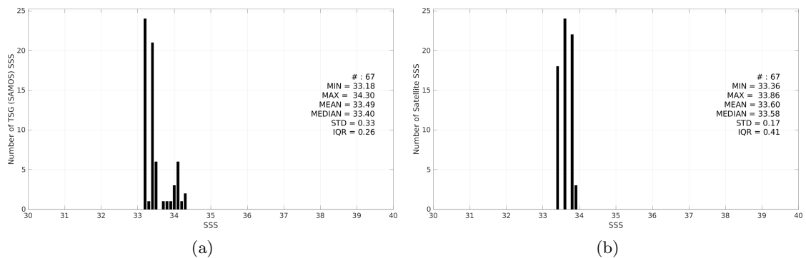
Figure 3: Histograms of SSS from TSG (SAMOS) (a) and Aquarius SSS L3 CAP v5 - 7-Day running (JPL) (b) considering all match-up pairs per bins of 0.1 over the Ganga and Brahmaputra river plumes Pi-MEP region and for the full satellite product period.
